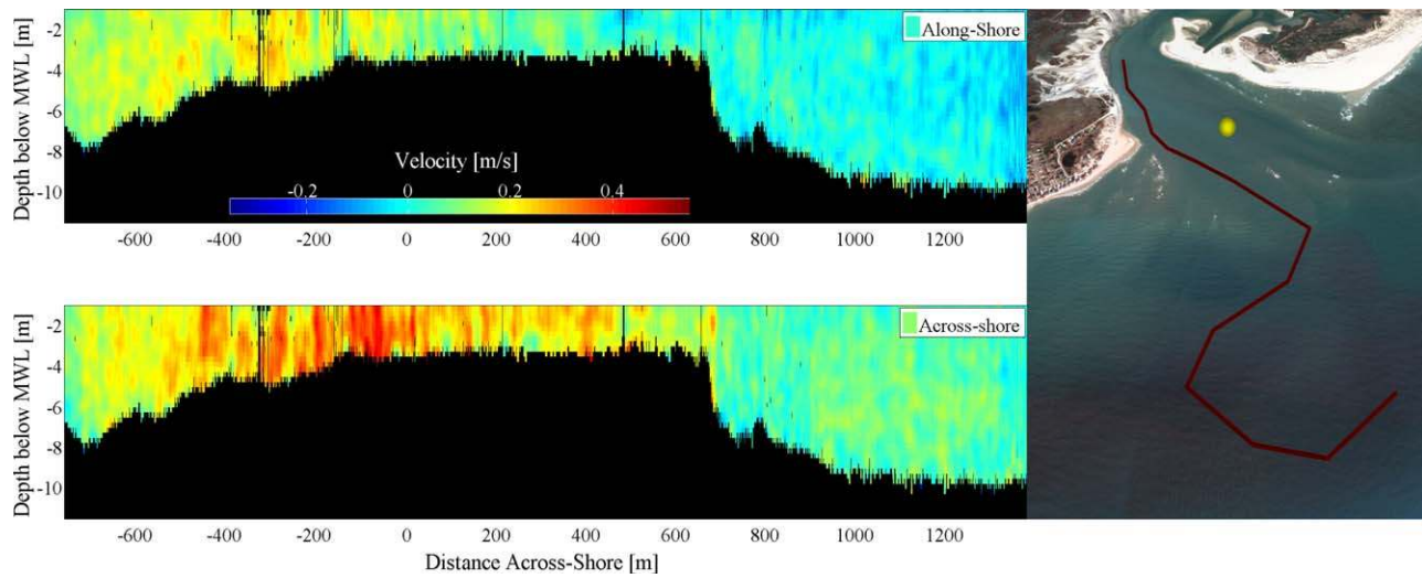
Figure 4. A sampling of the ADCP measured current profiles as SPEG crossed the NRI shoals. This data were taken from Run 13. Shown is the two-dimensional (top) alongshore and (bottom) across-shore flow velocity, where the color scale applies to both figures. On the right, the corresponding SPEG GPS track, with the (0,0) marked in yellow.
