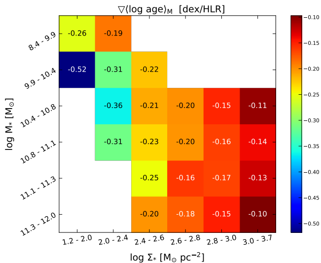
Fig. 13. Visual representation of Table 3 of the mass-weighted age gradients \nabla\langle\log \text{age}\rangle_M (dex/HLR) estimated over the inner 1 HLR for all galaxies as a function of both M_\star and \Sigma_\star .
