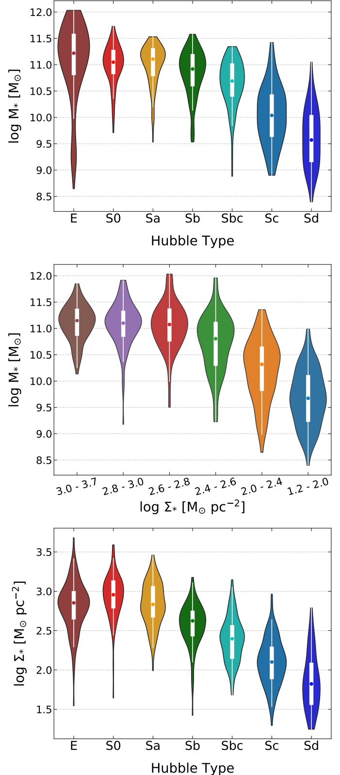
Fig. 1. Violin plots of the stellar masses for each Hubble type (upper panel), stellar masses for each stellar mass surface density bin (middle panel), and stellar mass surface density for each Hubble type (bottom panel). Its corresponding box plot showing the interquartile range is plotted inside each violin plot. The inner dot in the box plot represents the median of the distribution. The values of the stellar mass surface density were obtained at 1 HLR (see Sect. 3.3). The width of the “violins” are scaled by the number of observations in each bin.
