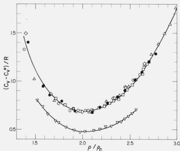
FIGURE 6. Reduced specific heats versus reduced density for CH_4 (●), F_2 (◇), O_2 (Δ), Kr (□), Ar (○), and Ne (▽).
