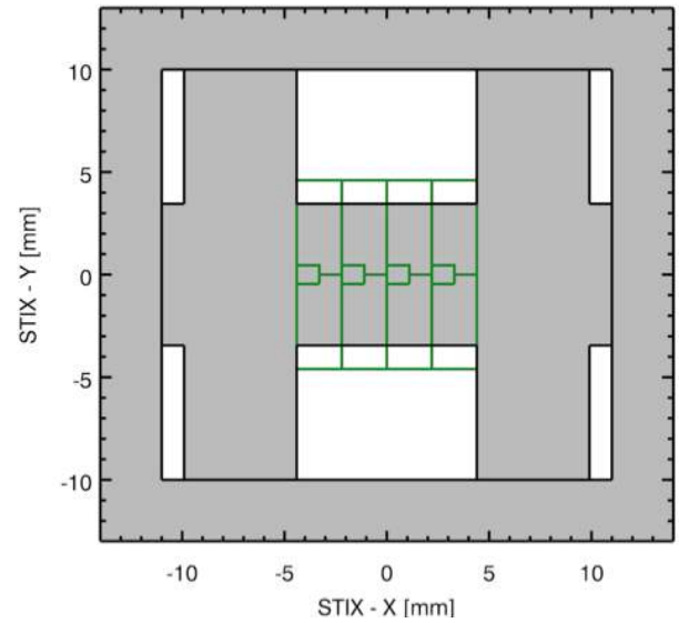
Fig. 9. Pattern of large apertures on the front grid for the CFL subcollimator. Its X-ray shadow (gray) is shown superimposed on the detector pixels (green) for an on-axis source. Different source locations can be visualized by shifting the detector relative to the mask.
