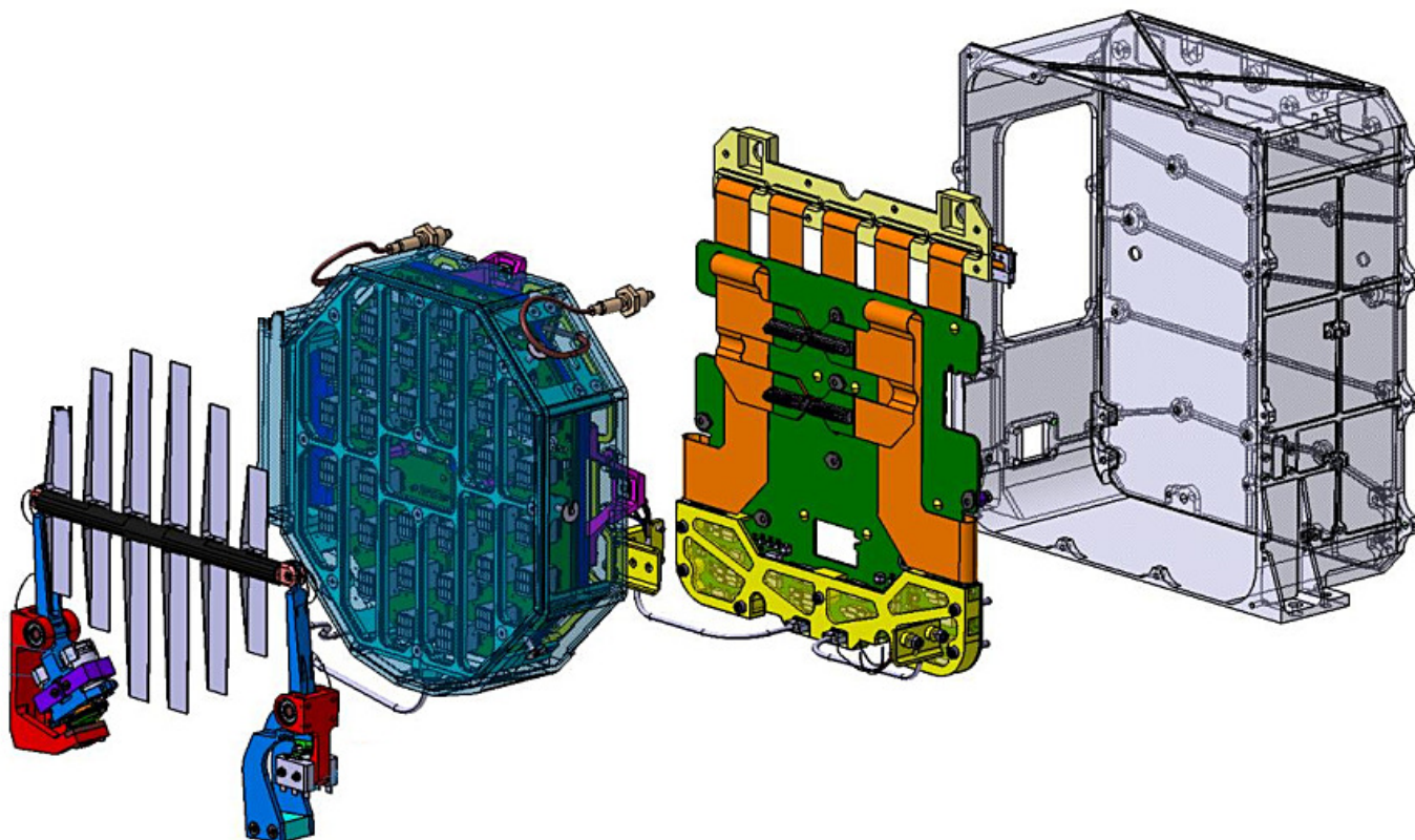
Fig. 11. Design of the Detector Box ( left to right ): the mechanical attenuator, the cold unit containing 32 Caliste-SO hybrids, the back-end electronics board with flex cable connections, and the housing. Not shown is the DEM entrance window to the left of the attenuator.
