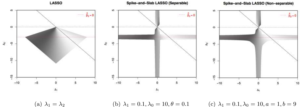
Figure 4: Plots of the feasible regions for \Theta under the LASSO penalty and the SSL penalty.
