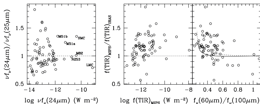
Figure 7. Comparison of the Spitzer and IRAS data for the LVL sample. The leftmost panel shows the ratio of Spitzer 24 \mu\text{m} and IRAS 25 \mu\text{m} data, and the right two panels compare the total infrared as measured from Spitzer and IRAS . The dotted line in the left two panels indicate a ratio of unity, whereas the solid and dotted lines in the rightmost panel indicate model predictions from Dale & Helou (2002) and Dale et al. (2001), respectively.
