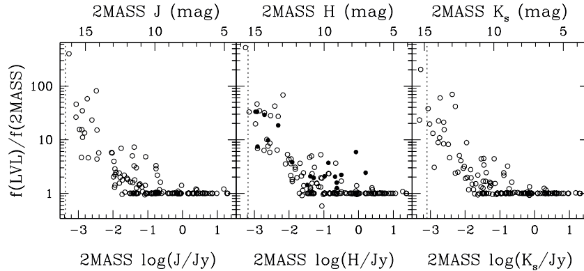
Figure 5. Comparison of near-infrared fluxes independently extracted from the 2MASS image archives using the apertures described in Section 4.2 with those from the 2MASS Extended Source Catalog. The filled circles are based on deep H band imaging of nearby galaxies with the 3.9 m Anglo–Australian Telescope (Kirby et al. 2008). The vertical dotted lines indicate the 2MASS 10\sigma point-source detection limits.
