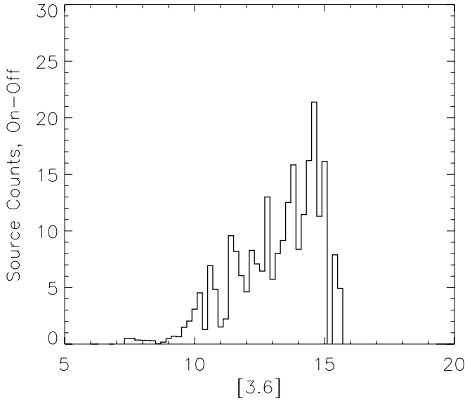
FIG. 20.— Top : Differential source counts at 3.6\ \mu\text{m} for the “core” cluster region of IC 5146. The solid line shows the counts for the combination of the two on-cluster areas; the dashed line shows the same for the sum of the two off-cluster regions; the smooth dash-dot line shows the prediction from the Wainscoat model for this direction in the Galaxy. Bottom : Difference in counts for the sum of the two on-cluster regions, i.e., on – off cluster counts normalized to the total of the two on-cluster areas in Fig. 18.
