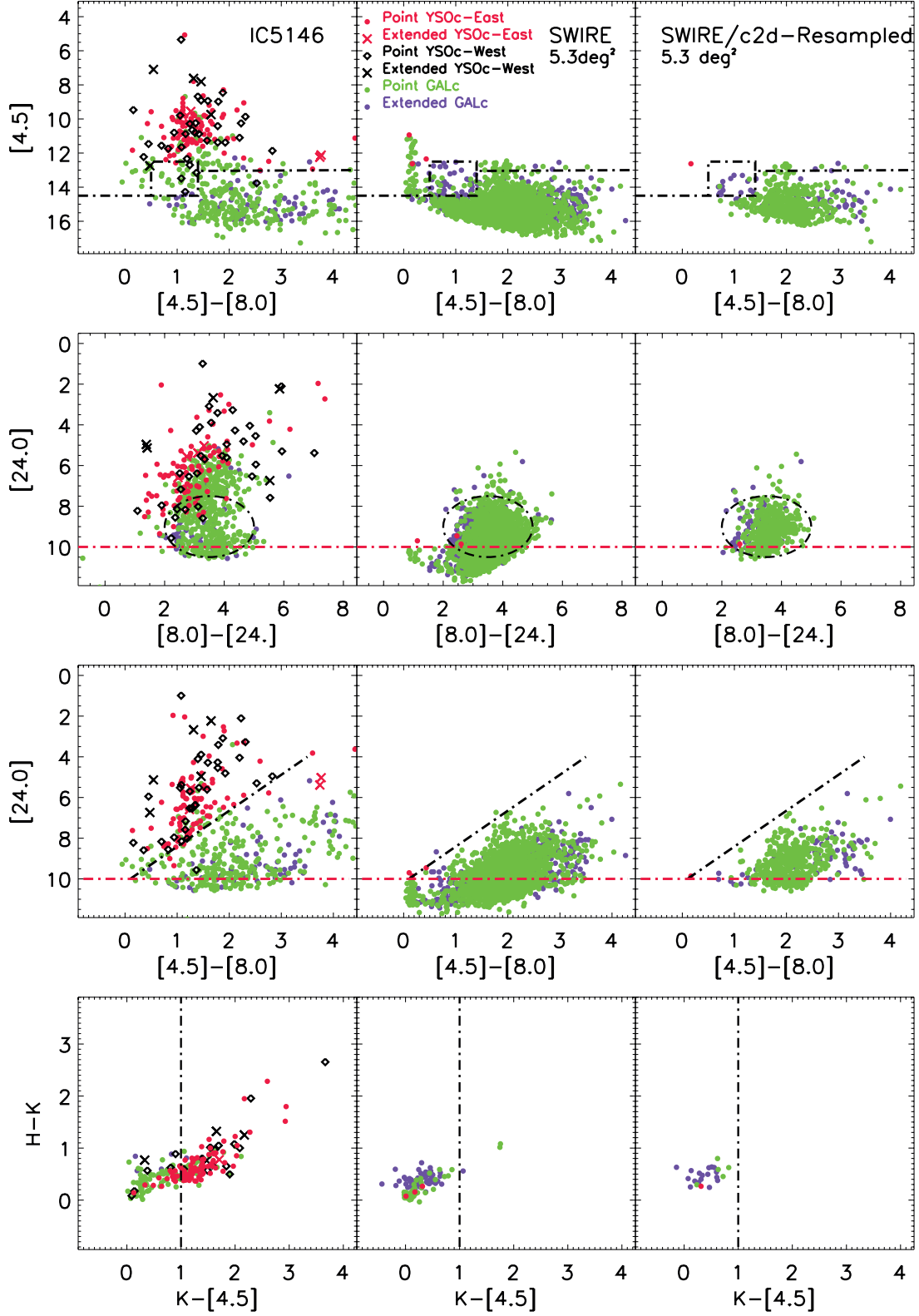
FIG. 4.—Color-magnitude and color-color diagrams for IC 5146 (left), full SWIRE (center), and trimmed SWIRE regions. The black dot-dashed lines show the “fuzzy” color-magnitude cuts that define the YSO candidate criterion in the various color-magnitude spaces. The red dot-dashed lines show hard limits, fainter than which objects are excluded from the YSO category.
