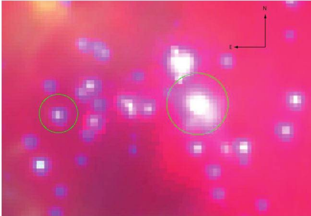
FIG. 8.—Area of 1' \times 1.5' in the center of the H II region showing the two objects with nonstellar images. BD +46 3474 is the object surrounded by nebulosity in the right half of the image and IfAHα 141 is the circled object in the left half of the image that is elongated north-south. In this image the 4.5 \mu\text{m} data are coded as blue, the 8.0 \mu\text{m} data as green, and the 24 \mu\text{m} data as red.
