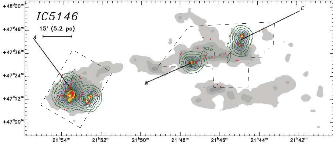
FIG. 23.—Volume density contours of the five-band YSOs in IC 5146 from Table 5 assuming a distance of 950 pc shown on top of extinction maps (Cambr sy 1999; gray scale ). The green contours indicate the volume densities corresponding to 12.5%, 25%, 50%, 200%, and 400% the criterion suggested by Lada & Lada (2003) of 1 M_{\odot} \text{pc}^{-3} ( 1 \times \text{LL03} ). The blue contours indicate the volume density corresponding to this criterion, and the yellow contours correspond to volume densities 25 times higher than this level. The red dots show the location of the YSOs in the cloud. The approximate areas of full five-band coverage are shown by the dashed lines, as well as shown exactly in Figs. 2 and 3.
