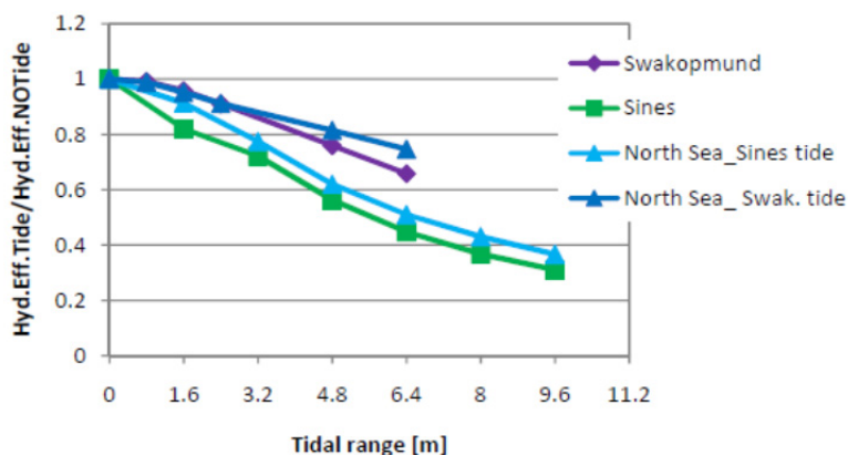
Figure 14. Decrease of hydraulic efficiency with increasing tidal ranges [19].
