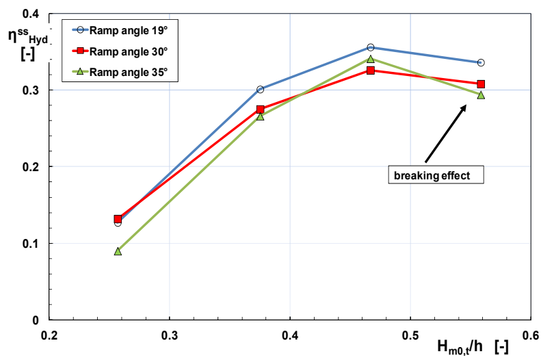
Figure 8. The effect of the outer ramp angle \alpha_r on the hydraulic efficiency [12] (SR = 1:15).
