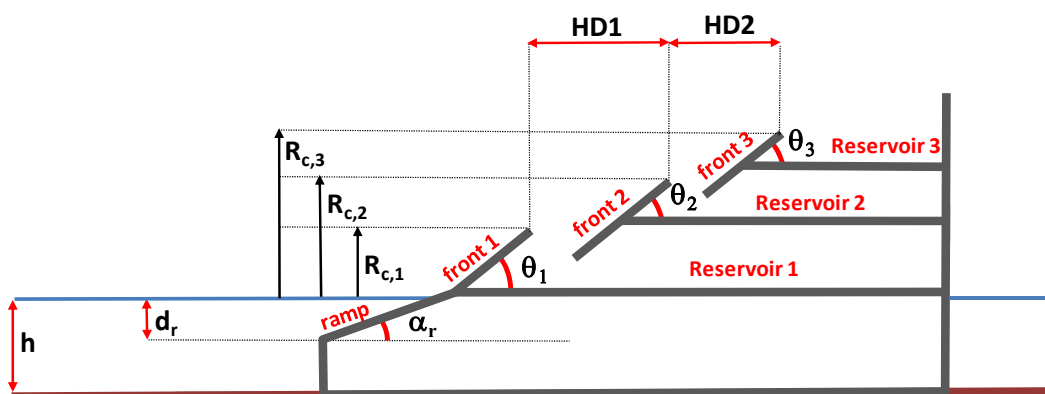
Figure 3. Definition sketch for a 3-level structure.
