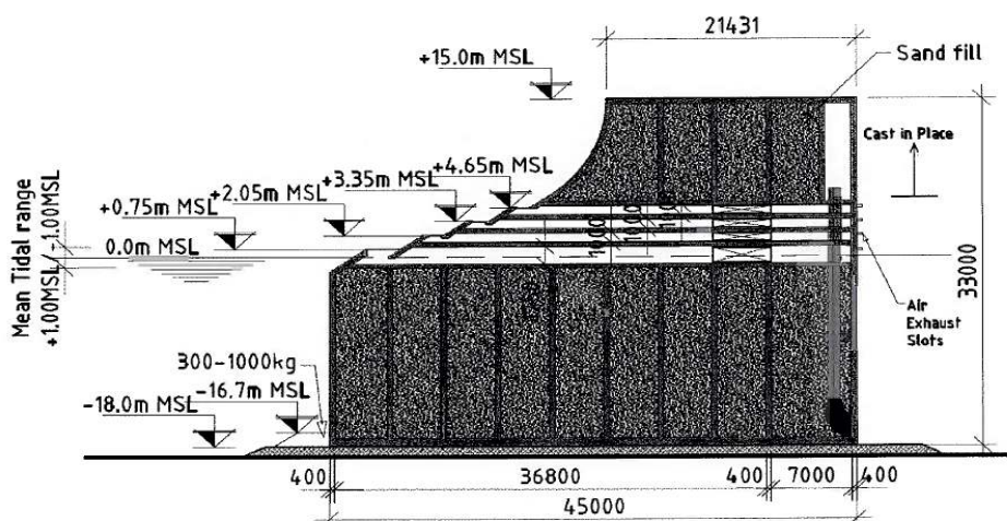
Figure 24. Section of the SSG-breakwater caisson at Sines.
