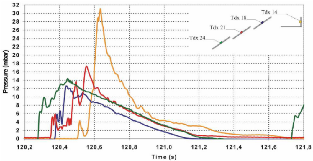
Figure 19. Wave shape under side attacks [11].
