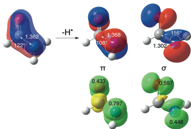
Fig. 2 HOMO/SOMO orbitals (red/blue surfaces) in formamide (left), \pi -radical ( cis -isomer, N1mag = 0 ), and \sigma -radical ( trans -isomer, N1mag = 0 ). The CNH bond angles, N–C bond lengths (in angstroms), spin distributions (NPA values), and spin SCF densities (green/yellow surfaces) for \pi - and \sigma -radicals have been calculated at UB3LYP/6-31G(d) level.
