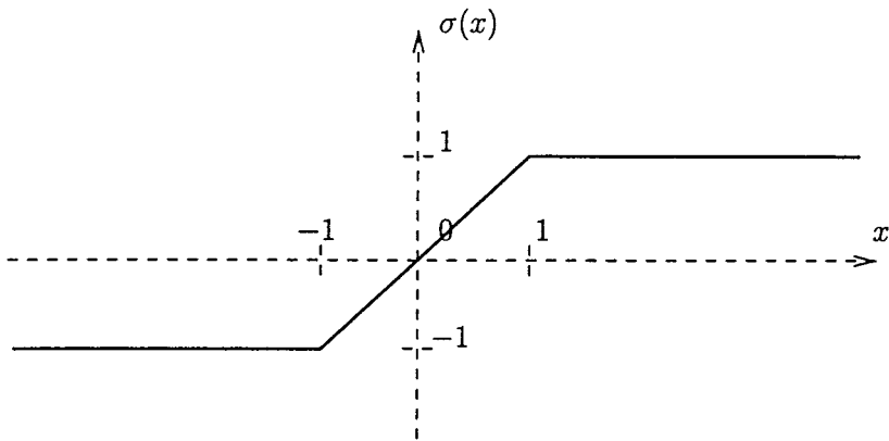
FIG. 1. Graph of the function \sigma .
