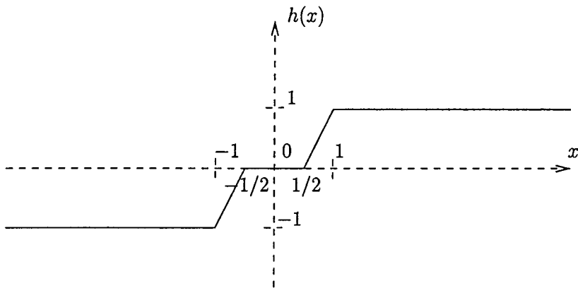
FIG. 2. Graph of the function h(x) = \sigma(2\sigma(x) - \sigma(2x)) .
