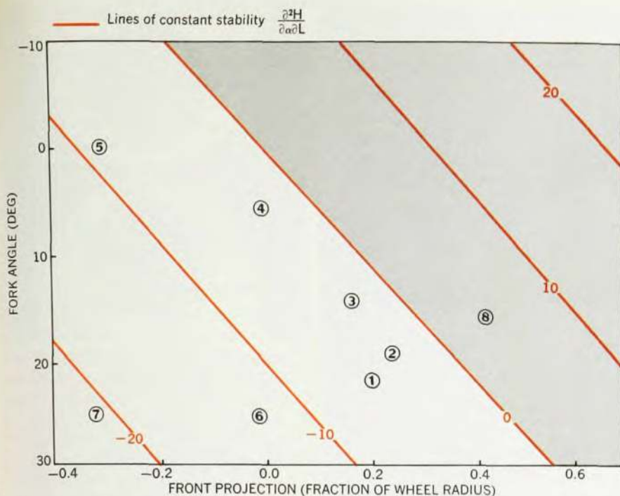
STABLE AND UNSTABLE BICYCLES. On this plot of fork angle versus front projection the d^2H/d\alpha dL lines are lines of constant stability. Grey area shows the unstable region. Point 1 is a normal modern bicycle; 2 is a racing bike. 3 and 4 are high-wheelers (or "penny-farthings") from the 1870's. Point 5 is an 1887 Rudge machine, and 6 is a Lawson "Safety" of 1879. Point 7 is URB III, and point 8, the only unstable bicycle, is of course URB IV. —FIG. 5
