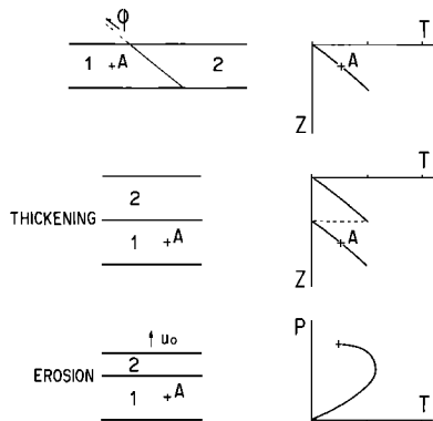
Fig. 2. Thickening by underthrusting. Movement along the thrust fault \phi brings instantaneously the "cold" unit 1 at the base of unit 2. Erosion restores the initial thickness. The uplift (P,T,t) path of a point A within unit 1 is presented, notice the temperature increase during uplift.
