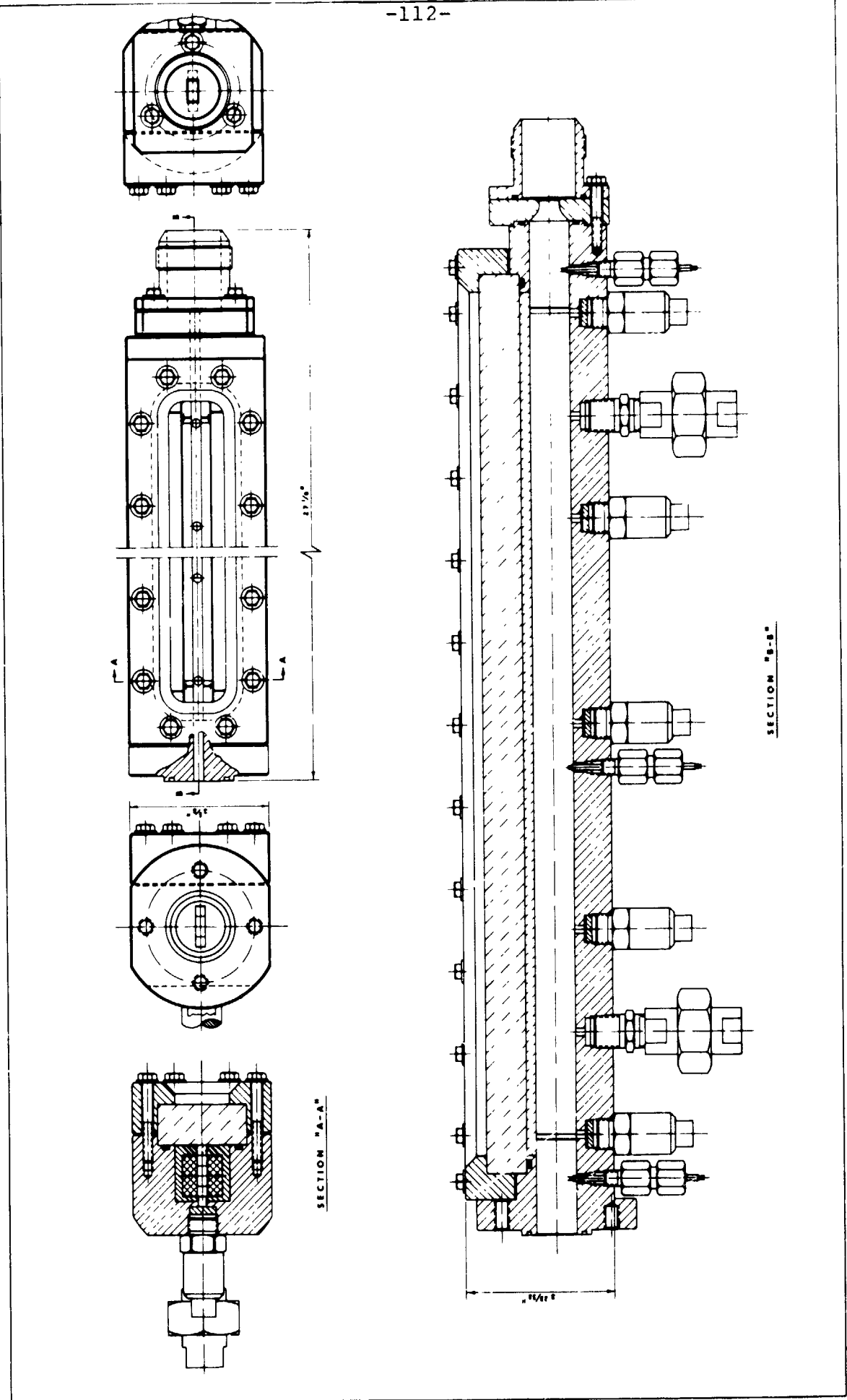
Fig. 10 Assembly drawing of the experimental window motor.
