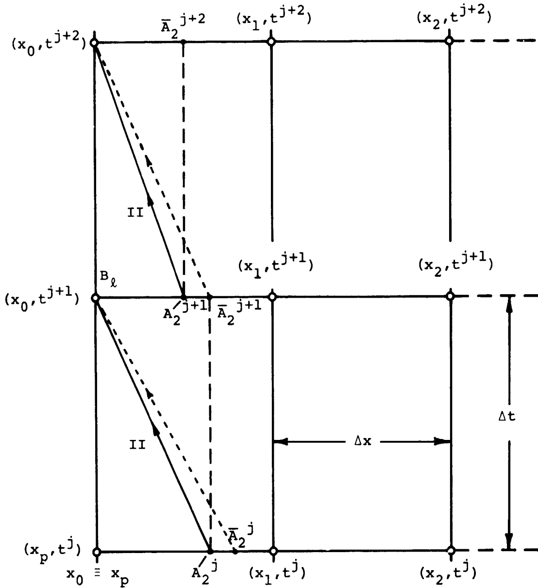
Fig. 8 Numerical calculation grid and characteristic directions at the left boundary of the calculated domain.
