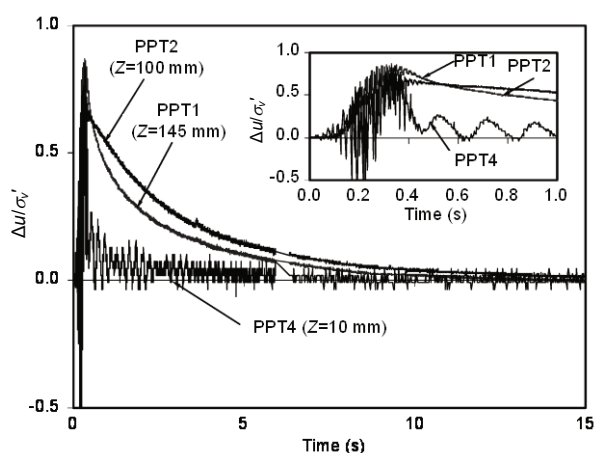
Fig. 27 Measured excess pore water pressure ratios in the bi-axial shaking test M2D-0.3 (Ng et al. , 2004b)
