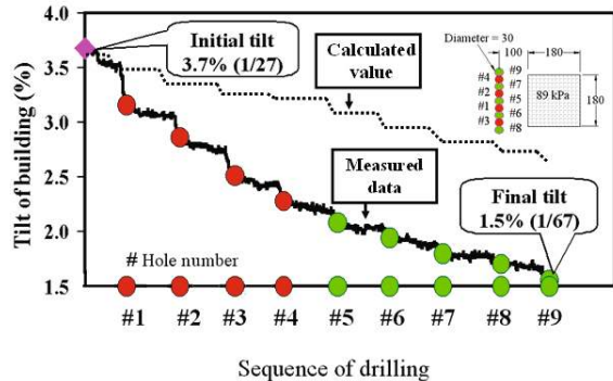
Fig. 9 Development of tilting of model building during soil extraction (all dimensions in mm, unless stated otherwise)
