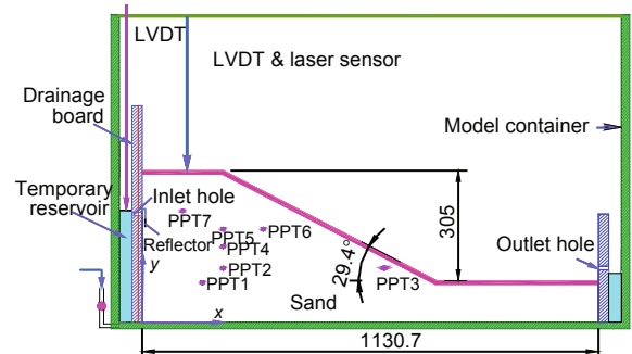
Fig. 19 Centrifuge model of a loose sand fill slope subjected to rising ground water table at 60g (unit: mm) (Zhang and Ng, 2003)
