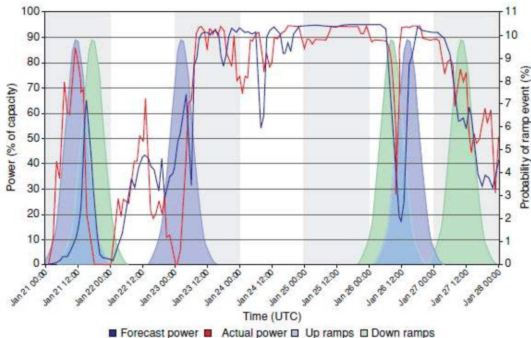
Figure 42: Visualisation of GL Garrad Hassan of ramp timing risk for up- and downramps. Source: [287]
