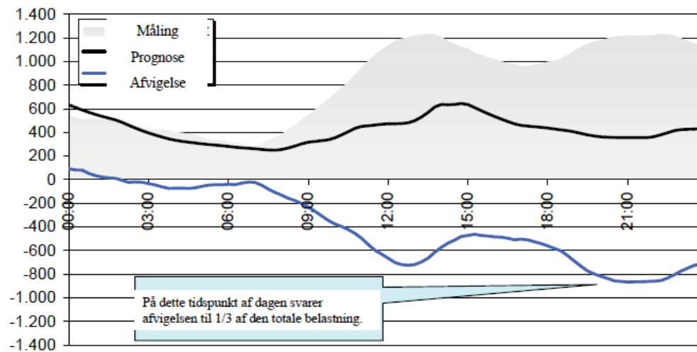
Figure 16: “The Bad”. Average energy per quarter hour on Oct 25, 2000. The forecast is from Oct 24, 11:00 hours. The Danish note says: “At this time of the day, the deviation corresponded to 1/3 of the total demand.”
