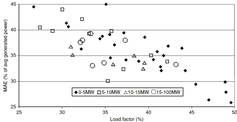
Figure 41: The MAE scaled with average generated power as a function of the load factor. Source: Lang and McKeogh [280].
