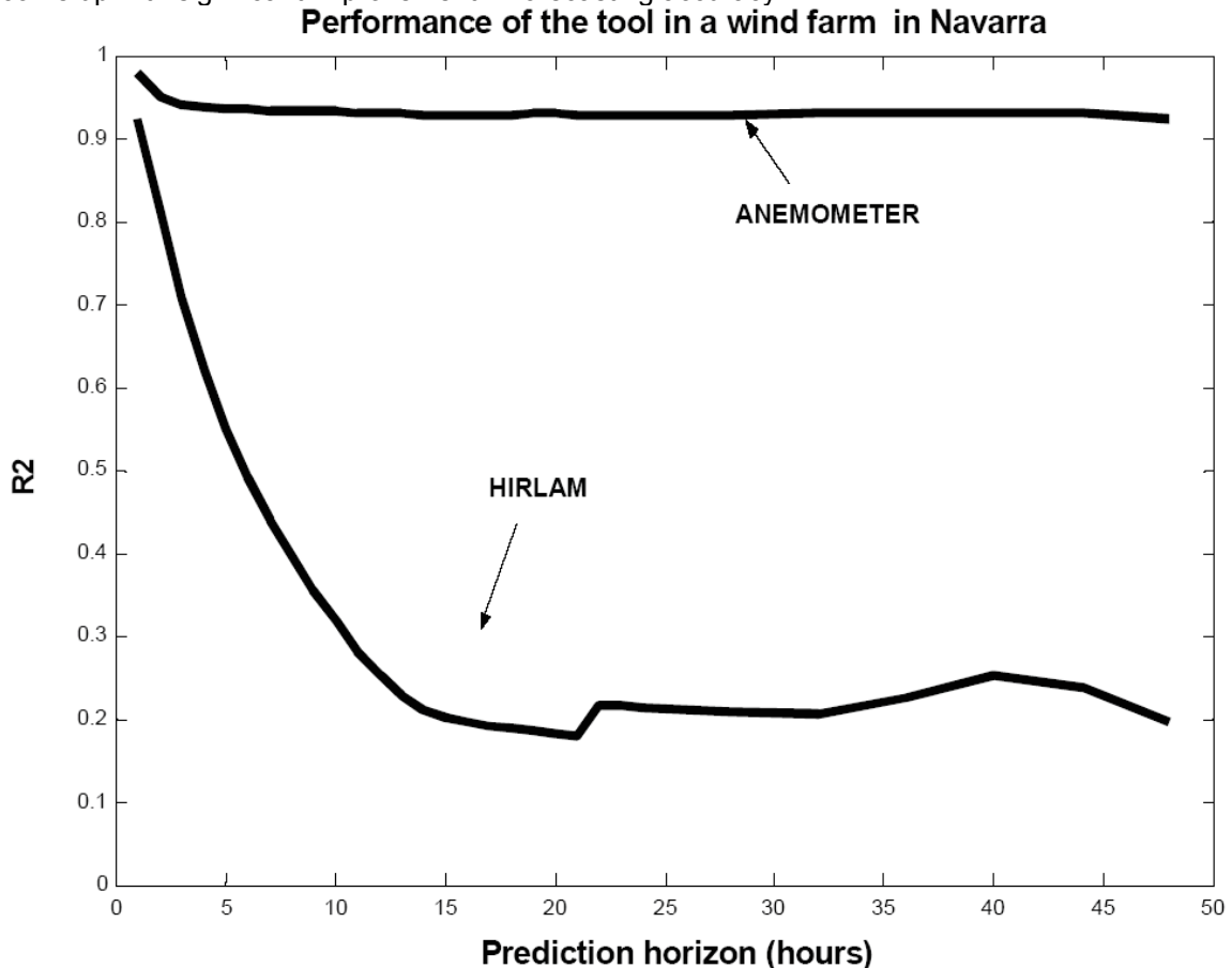
Figure 27: The error comes from the NWP. The figure shows the difference in degree of explanation between Sipleoico run with HIRLAM input (from an older version of the Spanish HIRLAM) and Sipleoico run with on-site wind speed input. Source: Sanchez et al. [125].
