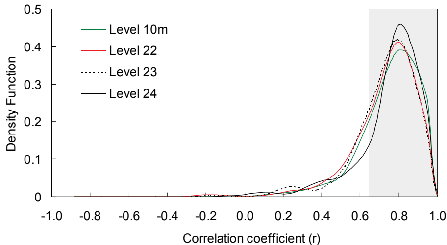
Figure 3: Distribution of correlation coefficient r(100) between Hirlam wind speed forecasts and measured wind park power. Source: Costello et al. [202]
