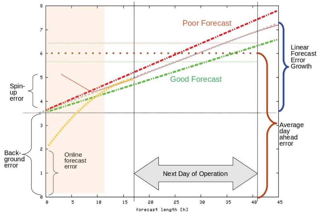
Figure 5: Typical errors introduced by the NWP. Source: Möhrlen [46].
