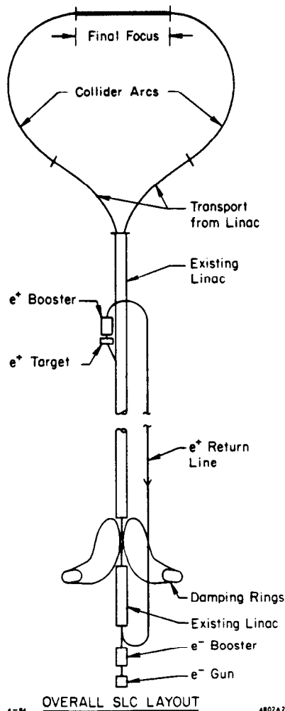
Fig. 1. Overall SLC Layout.
