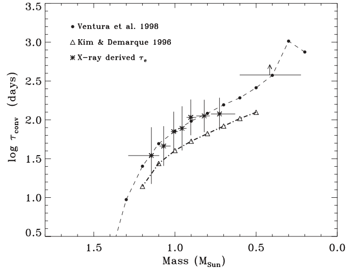
Fig. 10. Comparison between our empirically-determined \tau_e (asterisks), and theoretical predictions by Kim & Demarque (dash-dotted line) and by Ventura et al. (1998) (dashed line). Horizontal lines cover the mass ranges considered, while the asterisks are placed at the median of the masses of the corresponding bin.
