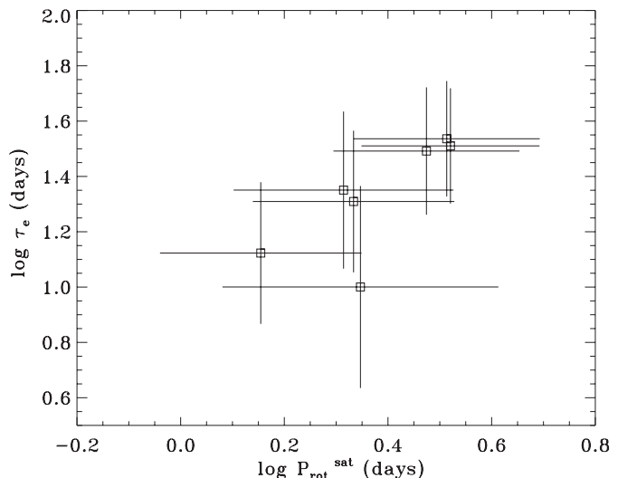
Fig. 12. Relationship between our empirical time scale and the rotation period at which the saturated X-ray emission is reached.
