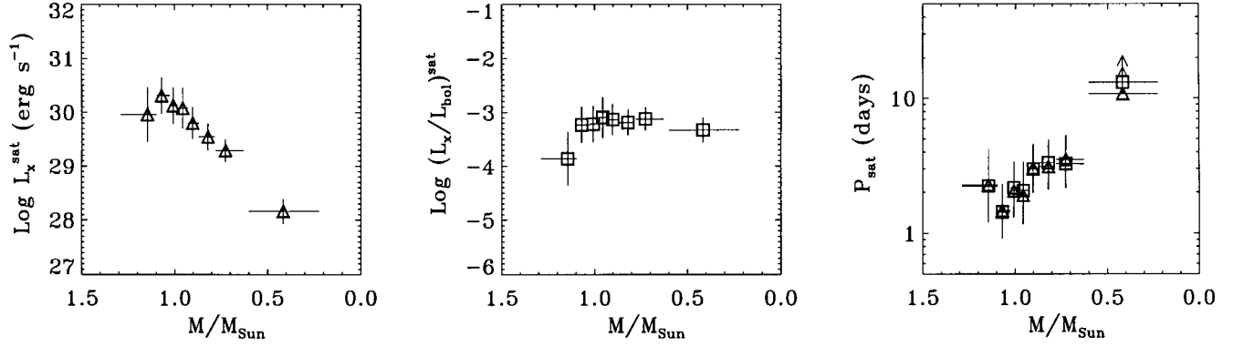
Fig. 7. Results of the fitting analysis reported in Table 3: the left and central panel show, respectively, the variation of L_x and L_x/L_{\text{bol}} saturation level with the stellar mass; the right panel shows variation of the rotation period at which saturation of L_x (triangles) and L_x/L_{\text{bol}} (squares) occurs vs. stellar mass. The horizontal segments indicate the ranges of the mass bins, with the vertical error bar (or lower limit) located at the median value of the masses for the stars in each bin.
