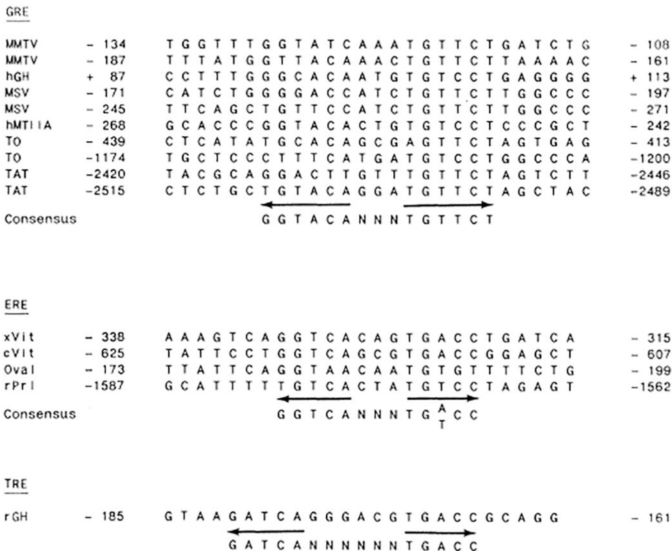
Fig. 1. Alignment of nucleic acid sequences in regions correspond to identified HREs (15–25). Numbering refers to nucleotide position relative to the start of transcription. Arrows indicate dyad axis of symme consensus sequence is derived from nucleotides conserved with a frequency of 50% or more. Specific references for HREs can be found in Fig. 2. GRE glucocorticoid response element; MMTV, mouse mammary tumor virus; hGH, human growth hormone; MSV, murine sarcoma virus; hMTIIA, human metallothionein; TO, tyrosine oxidase; TAT, tyrosine aminotransferase; ERE, estrogen response element; xVit, Xenopus vitellogenin; cVit, chicken vitellogenin; Oval, chicken ovalbumin; rPrI, rat prolactin; TRE thyroid hormone response element; and rGH, rat growth hormone.
