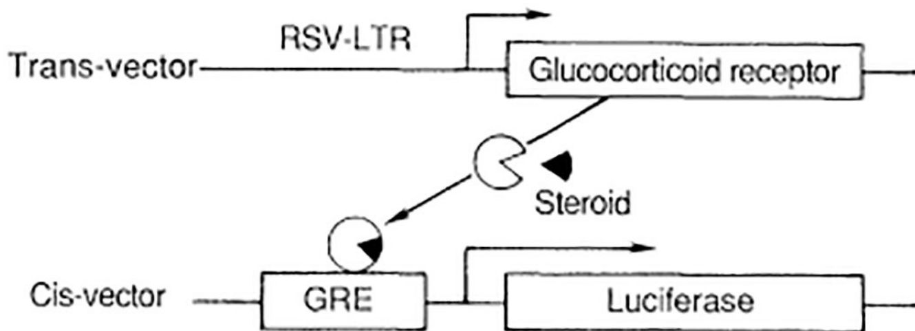
Fig. 3. The cotransfection assay. Cultured cells are transfected with the receptor cDNA in an expression vector (the trans-vector). The function of this transcription factor can be monitored by the activity of a reporter gene (the luciferase gene) linked to an appropriate hormone-responsive promoter. In this case, the promoter is from the MMTV virus carrying a GRE enhancer. The trans-vector encodes the hGR, shown combining with the steroid hormone (triangle).
