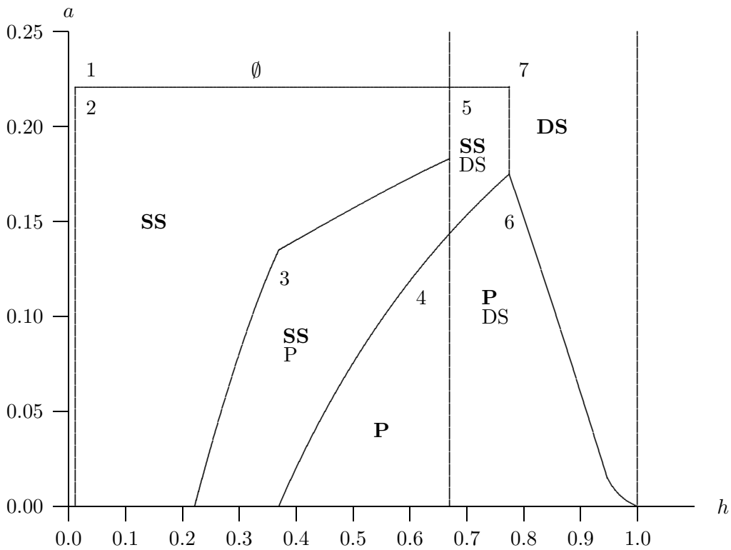
Figure 1: Pareto optimal equilibria
