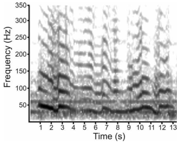
Figure 3. An exceptionally long duration rumble produced over a period of 13 s. Long rumbles, exceeding 2 s, were infrequently produced and constituted only 30% of the total number of recorded rumbles. This rumble shows a net frequency modulation of 19 Hz when the onset dominant frequency is compared to the dominant frequency at the end of the rumble. Noise generated by external pumps was present in the constant 30 and 60 Hz frequency bands; the 60 Hz band obscures some of the rumble harmonics. A recording of this sound is available as supplementary material online.
