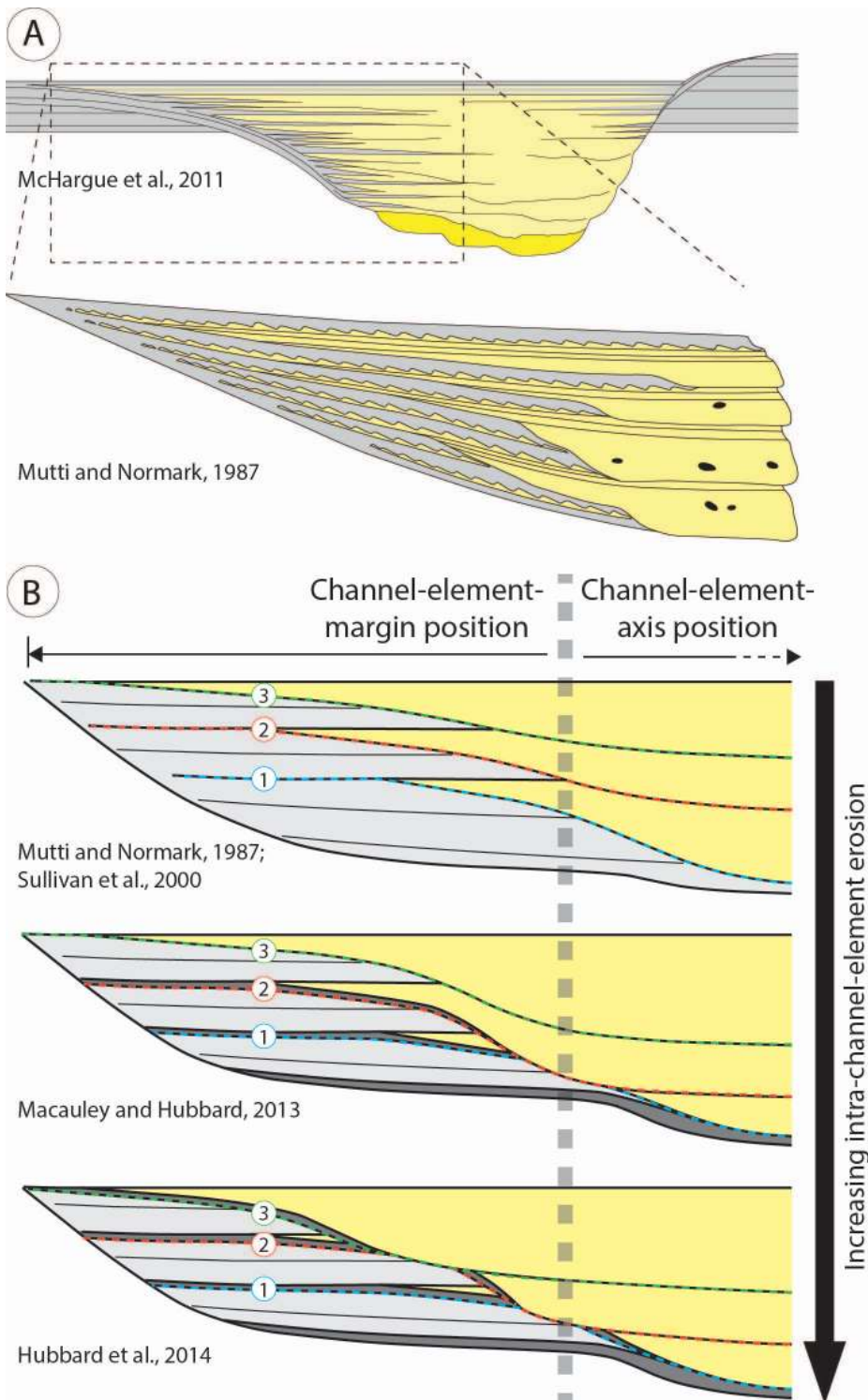
FIG. 1.—Channel-element stratigraphic architecture. A) Channel elements highlighting the basal erosion surface overlain by a fill that includes numerous erosion surfaces (modified from Mutti and Normark 1987; McHargue et al. 2011). Coarse-grained amalgamated sandstone beds transition laterally to thinner bedded sandstone and siltstone. B) Half channel widths that show variable configurations of internal erosion surfaces (i.e., secondary channel-form surfaces labeled 1–3), largely differentiated by depth of incision. The degree of incision controls the nature of interfingering amongst siltstone and thick-bedded sandstone at the transition between the element axis and margin. Approximate scales of sketches are 15–25 m thick (maximum) and 100–200 m wide.
