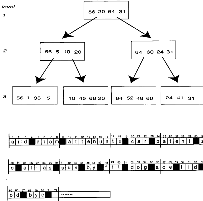
FIG. 3. An example of B-tree-like layout (upper part) and its input string set \Delta (lower part). Set \mathcal{K} = \{\text{'ace'}, \text{'aid'}, \text{'atlas'}, \text{'atom'}, \text{'attenuate'}, \text{'by'}, \text{'bye'}, \text{'car'}, \text{'cod'}, \text{'dog'}, \text{'fit'}, \text{'lid'}, \text{'patent'}, \text{'sun'}, \text{'zoo'}\} is obtained by sorting \Delta . The strings in \mathcal{K} are stored in the B-tree leaves by means of their logical pointers 56, 1, 35, 5, 10, . . . , 31.
