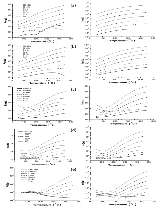
Fig. 5. Variation of real and imaginary parts of dielectric constant with temperature at different frequencies for (1-x)\text{Ba}(\text{Fe}_{1/2}\text{Nb}_{1/2})\text{O}_3-x\text{BaTiO}_3 ceramics (a) x = 0 , (b) x = 0.25 , (c) x = 0.50 , (d) x = 0.75 and (e) x = 1 .
