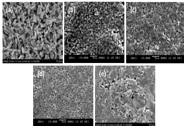
Fig. 3. Scanning electron micrographs of (1-x)\text{Ba}(\text{Fe}_{1/2}\text{Nb}_{1/2})\text{O}_3-x\text{BaTiO}_3 ceramics (a) x = 0 , (b) x = 0.25 , (c) x = 0.50 , (d) x = 0.75 and (e) x = 1.0 .
