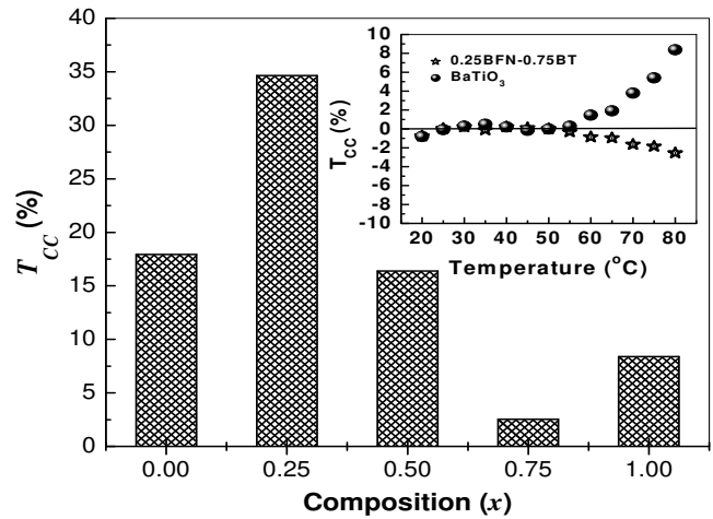
Fig. 6. Compositional variation of T_{CC}(\%) of (1-x)\text{Ba}(\text{Fe}_{1/2}\text{Nb}_{1/2})\text{O}_3-x\text{BaTiO}_3 ceramic. Inset: Variation of T_{CC}(\%) with temperature for x = 0.75 and 1.0 .
