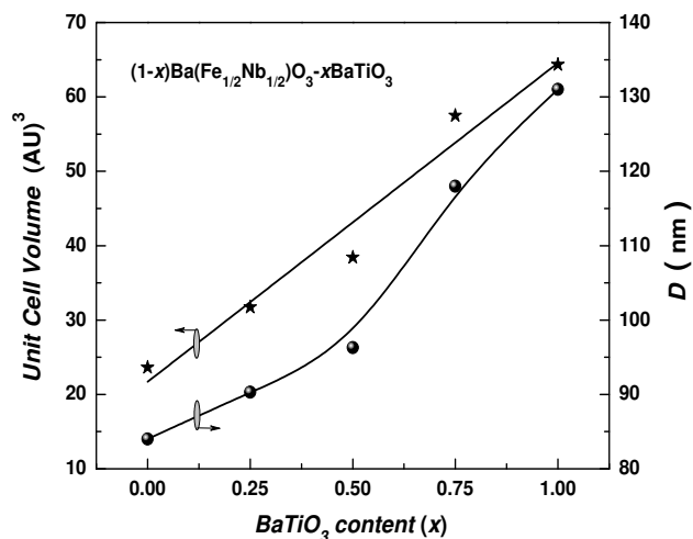
Fig. 2. Variation of apparent particle size and unit cell volume with composition of (1-x)\text{Ba}(\text{Fe}_{1/2}\text{Nb}_{1/2})\text{O}_3-x\text{BaTiO}_3 ; x = 0, 0.25, 0.50, 0.75 and 1.0 ceramics.
