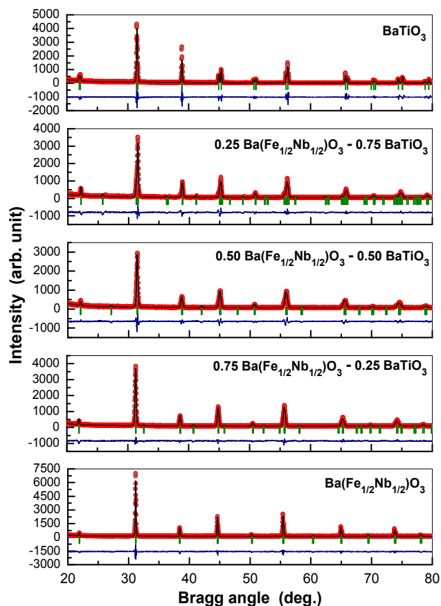
Fig. 1. Rietveld refined pattern of (1-x)Ba(Fe_{1/2}Nb_{1/2})O_3-xBaTiO_3 ; x = 0, 0.25, 0.50, 0.75 and 1.0 ceramics. Symbols represent the observed data points and the solid lines their Rietveld fit.
