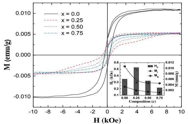
Fig. 7. Magnetization curves for (1-x)\text{Ba}(\text{Fe}_{1/2}\text{Nb}_{1/2})\text{O}_3-x\text{BaTiO}_3 ; x = 0, 0.25, 0.50 and 0.75 ceramics at room temperature. Inset: Compositional variation of H_C , M_r and M_S .
