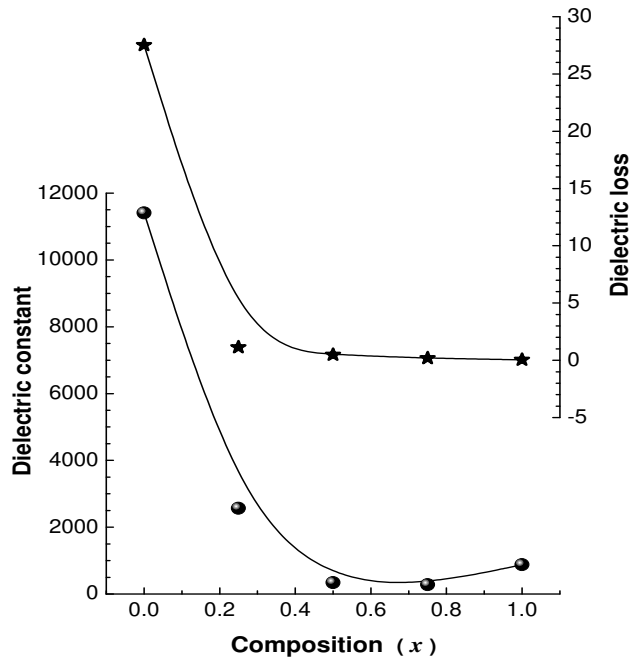
Fig. 4. Compositional variation of dielectric constant and dielectric loss of (1-x)\text{Ba}(\text{Fe}_{1/2}\text{Nb}_{1/2})\text{O}_3-x\text{BaTiO}_3 ceramics.
