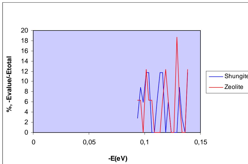
Figure 4. The distribution ( \% , (-Evalue)/(-Etotal) value) of water molecules in water solution of shungite/zeolite according to energies of hydrogen bonds ( -Evalue ) to total result of hydrogen bonds energy
