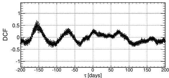
Figure 14. DCF between derived for the \gamma -ray and X-ray bands. Positive values of ‘ \tau ’ correspond to flux variations in the \gamma -ray band lagging flux variation in the X-ray band.
