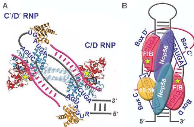
Figure 6. Class C/D sno(s)RNP architecture. (A) The archaeal C/D sRNP assembles with a copy of each core C/D proteins (colored as in Figures 4 and 5) at both the C/D and C'/D' RNA motifs (blue) of the sRNA (grey), and guides methylation of a RNA nucleotide (pink) at each site. The observed quaternary structure of the fibrillarin-Nop5 complex would position two fibrillarins catalytic sites (yellow star) ~80 Å apart. In contradiction to this observation, the distance between catalytic C/D and C'/D' sites of the sRNAs is highly conserved and only ~25–35 Å, suggesting the coiled-coiled interactions (transparent coloring) of Nop5 may be reorganized and/or disrupted in the fully assembled sRNP. (B) The C/D snoRNP is proposed to assemble into a pseudo-symmetric architecture. In contrast to the archaeal L7Ae protein, the Snu13/15.5 kDa protein appears to bind solely at the C/D site of the snoRNA. The Nop5 paralogs, Nop56 and Nop58, recognize the C and C' Box elements, respectively, while a copy of fibrillarins (Fib) interacts with each D and D' Box, consistent with its role in the catalytic center (yellow star).
