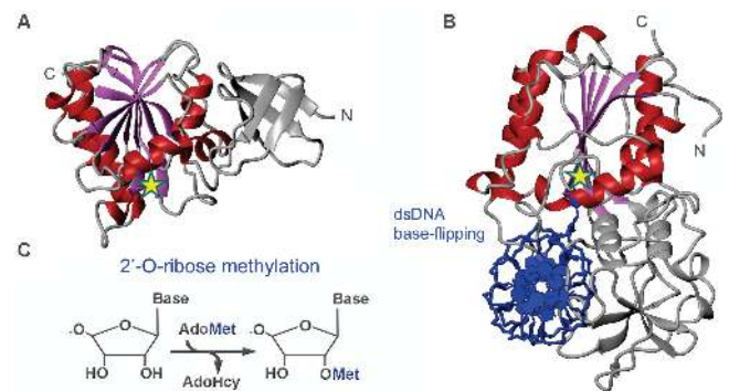
Figure 2. The conserved C/D methyltransferase fibrillarin. Crystal structure of (A) the archaeal fibrillarin (1FBN) and (B) of the double-stranded DNA methyltransferase HhaI (1MHT). The catalytic domains are colored according to their secondary structural elements (red: \alpha -helices; violet: \beta -strand; grey: variable regions). S -adenosyl-methionine (AdoMet) binds at a conserved site (yellow star) of these related enzymes. Structural details of fibrillarin interaction with the sno(s)RNA-target RNA complex are unknown. HhaI flips out the nucleobase to be modified in dsDNA (blue). (C) Fibrillarin catalyzes the ribose-2'-O-ribose methylation of its RNA substrates by converting AdoMet to S -adenosylhomocysteine (AdoHcy).
