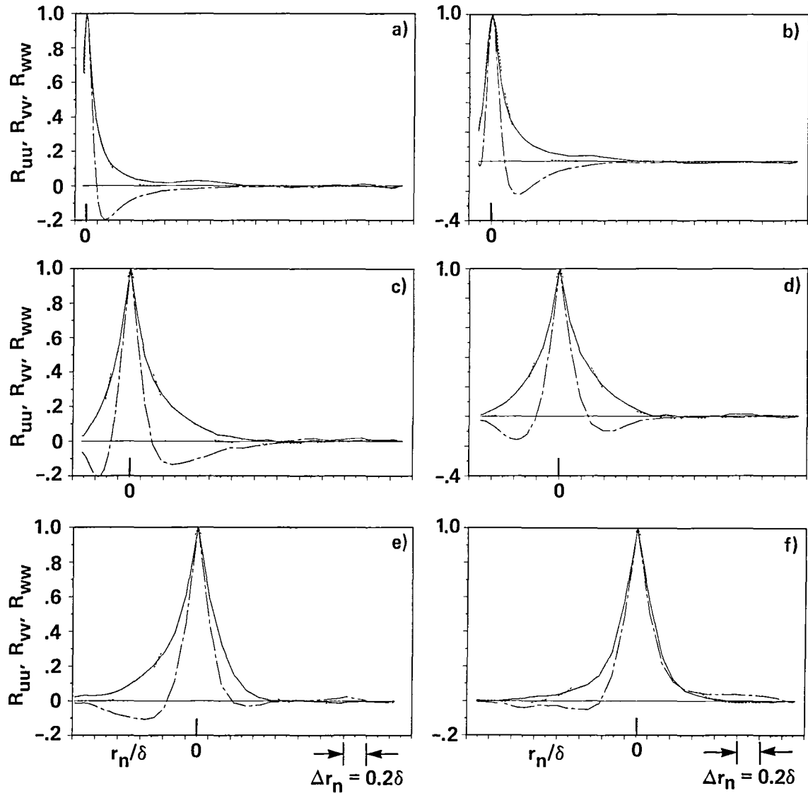
Figure 7. Two-point correlations of the velocity components with the direction of separation in (x,y) -plane and inclined at 135^\circ to the wall. — R_{uu} ; ---- R_{vv} ; -.- R_{wv} . See the caption of figure 6 for the y -location of the fixed point for each figure.
