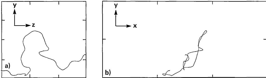
Figure 15. Close-up of the hairpin-like structure in figure 14. (a) 2-D end-view ,the spanwise, z , extent of the figure is 1.1\delta(700\nu/u_r) ; (b) 2-D side view ( (x,y) -plane ), the streamwise, x , extent of the figure is 2.15\delta(1380\nu/u_r) .
