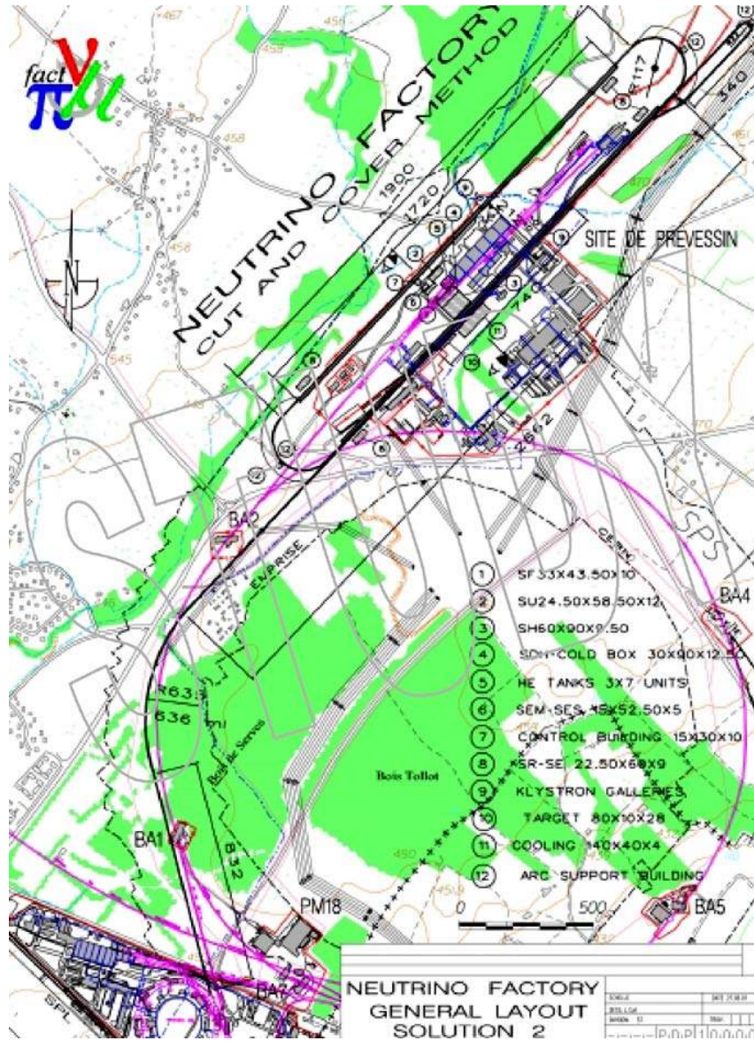
Fig. 2.2: Possible layout of a Neutrino Factory on the CERN site. The SPL and the accumulator ring can be seen at the lower left on the Meyrin site, while target station, cooling, recirculating linacs, and decay ring could be situated on the Prévessin site.
