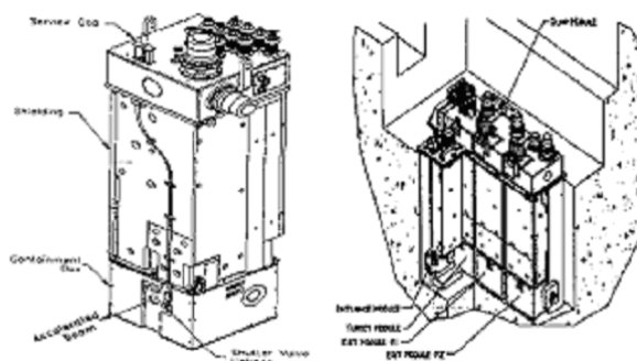
Fig. 4.6 ISAC target plugs
