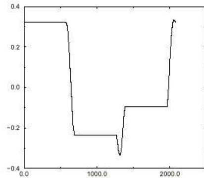
Fig. 7.4 Roll angle y along the circumference of the muon storage ring
