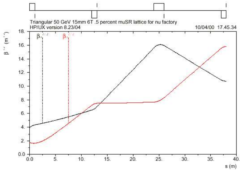
Fig. 7.7 Optical functions of the matching cells
