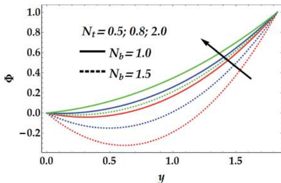
Fig. 5 Concentration distribution for various values of N_t and N_b at We = 0.01 , M = 1 , G_{rT} = 0.5 , G_{rF} = 0.6 , \gamma = 0.1 , and n = 2 .
