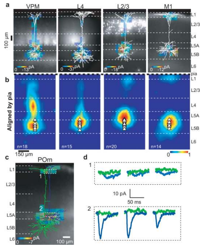
Figure 3. Subcellular distribution of inputs onto L5B pyramidal neurons
