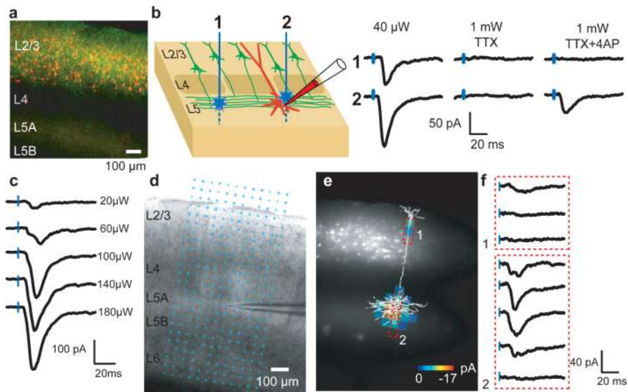
Figure 1. Subcellular Channelrhodopsin-2-Assisted Circuit Mapping (sCRACM)
