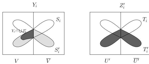
Figure 6: Allocation scheme 4.
