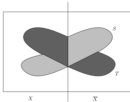
Figure 1: Algorithm 1.
