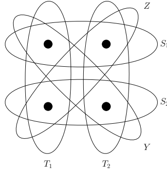
Figure 2: A half-integral solution.
