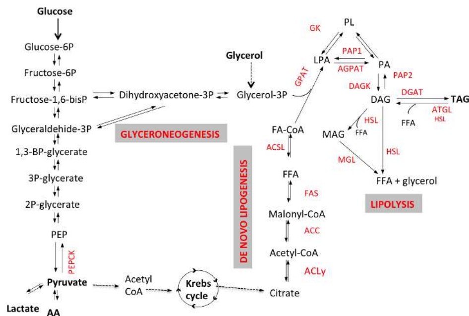
Figure 1. Schematic representation of lipolytic and lipogenic pathways. Triacylglycerol (TAG) synthesis requires the activation of free fatty acids (FFA) into Acyl-CoA by enzyme acyl-CoA synthetase. FFA-CoA and G3P are transformed via acylation, by glycerol-3-phosphate acyltransferase (GPAT) and acylCoA acylglycerol-3-phosphate acyltransferases (AGPAT), to phosphatidic acid (PA); then, after a dephosphorylation by phosphohydrolase (PAP2), diacylglycerols (DAG) are formed. Diacylglycerol acyltransferase (DGAT) catalyzes the conversion of DAG into TAG. In the adipocyte, G3P might come either from glycolysis or from non-carbohydrate substrates via the enzyme phosphoenolpyruvate carboxykinase (PEPCK), through a process named glyceroneogenesis. In the liver G3P can also be synthesized from plasma glycerol. De novo fatty acids synthesis (also referred to as de novo lipogenesis or DNL) occurs in the cytoplasm of various cells (e.g., adipocytes and hepatocytes) where citric acid is converted to acetyl-CoA by ATP-citrate lyase (ACL) and subsequently to malonyl-CoA by acetyl-CoA carboxylase (ACC). DNL occurs mainly in the liver, but it might occur in adipose tissue as well, although with low rates. This process requires the two enzymes ATP-citrate lyase (ACL), acetyl-CoA carboxylase (ACC) and the multi-enzymatic complex fatty acid synthase (FAS). G3P can be synthesized directly from non-carbohydrate substrates such as pyruvate, lactate or amino acids in oxaloacetate, that is converted to G3P either directly from phosphoenolpyruvate (PEP), via the key enzyme phosphoenolpyruvate carboxykinase (PEPCK), or through synthesis of dihydroxyacetone (DHA). TAG catabolism ( i.e. , lipolysis) involves several lipases, adipose triglyceride lipase (ATGL), hormone-sensitive lipase (HSL) and monoacylglycerol lipase (MGL) and produces the release of three free fatty acids (FFA) and one glycerol molecule.
