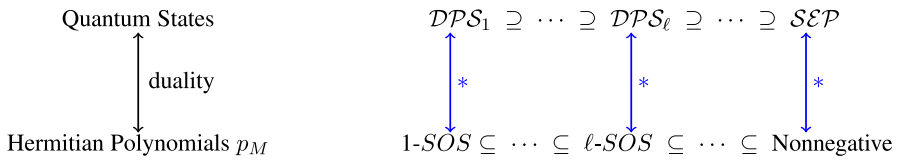
Fig. 1 A summary of the duality relations between the DPS hierarchy and sums of squares. The notation \ell -SOS is a shorthand for \|y\|^{2(\ell-1)} p_M is a real sum-of-squares
