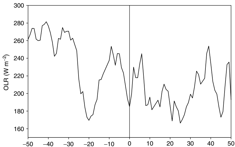
Figure 7. Daily mean OLR in the box 70-95^\circ E , Eq- 15^\circ N for 1998 with respect to the date of MOK
