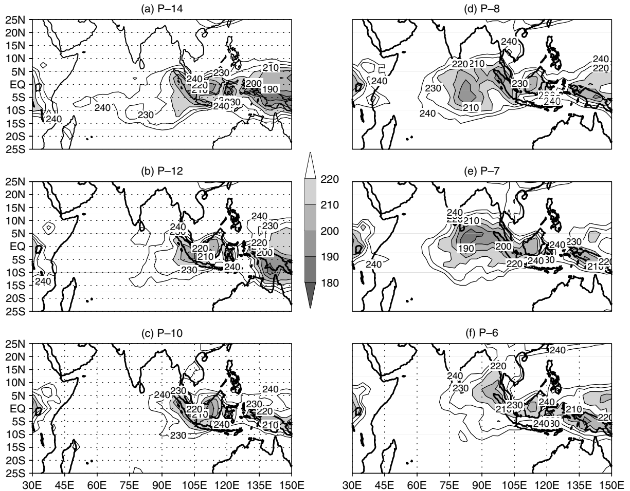
Figure 2. (a–f) Pentad mean OLR in W/m^2 for pentads (P – 14, P – 12, P – 10, P – 8, P – 7, P – 6, P – 5, P – 4, P – 3, P – 2, P – 1 and P0) as a composite of 9 years; 1979, 1982, 1984, 1986, 1987, 1990, 1993, 1995 and 1996. Only contours of 240 W/m^2 and less at intervals of 10 W/m^2 are shown. Contours below 220 W/m^2 are shaded up to 180 W/m^2 . MOK is at the middle of 0-Pentad. Pentad number is marked on top of each figure
