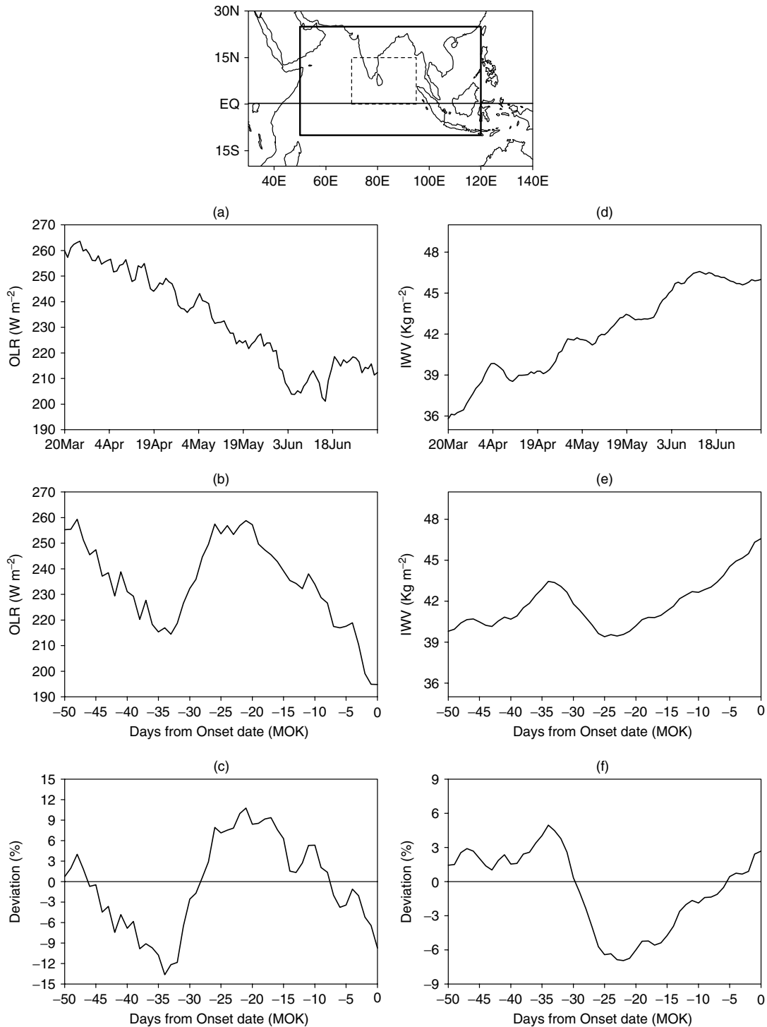
Figure 1. Twenty-year average by calendar date of (a) OLR (in W m^{-2} ) and (d) IWV (in kg m^{-2} ) for 1979–1998 of the inner box ( 70^{\circ} – 95^{\circ} E, Eq– 15^{\circ} N), marked in the inset figure by the dotted lines. Composite mean (b) OLR and (e) IWV of the inner box for the 9 years; 1979, 1982, 1984, 1986, 1987, 1990, 1993, 1995 and 1996 with respect to MOK as 0. Composite percentage departure of (c) OLR and (f) IWV for the above 9 years from the average for 20 years (1979–1998). The outer box marked by thick line is bounded by 50^{\circ} – 120^{\circ} E and 10^{\circ} S– 25^{\circ} N
