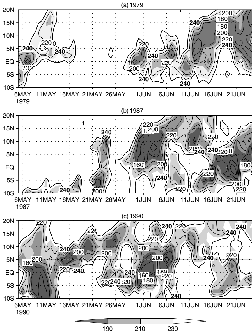
Figure 15. Hovmuller of OLR averaged along the longitudes 65°E–80°E. Contours less than 240 W/m 2 at intervals of 20 W/m 2 are shown. Contours are shaded from 190 to 230 W/m 2 . Thick line represents the 240 W/m 2 contours
