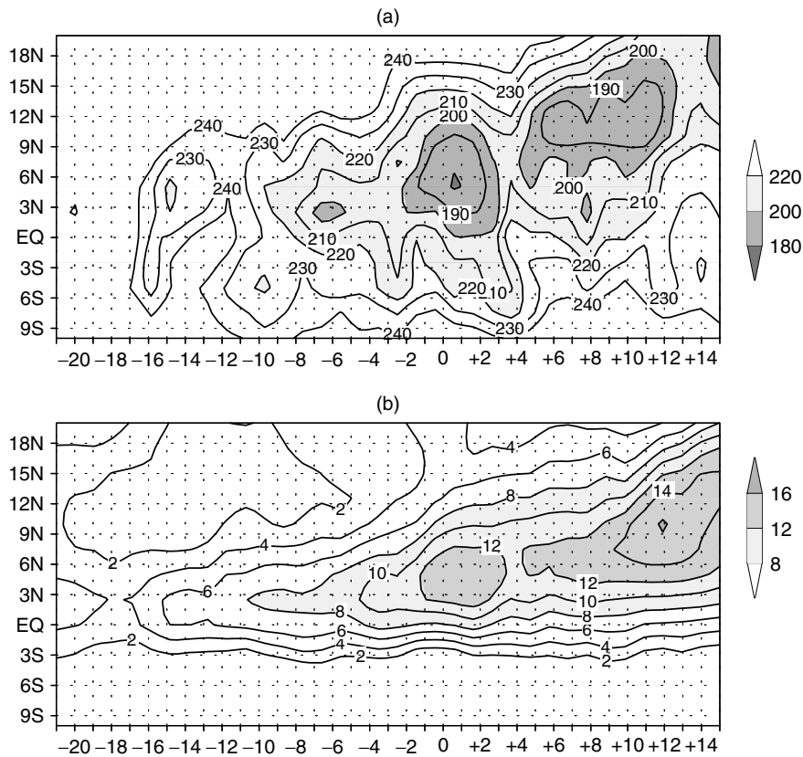
Figure 6. Composite (9-year) Hovmuller diagrams of (a) OLR in W/m^2 and (b) 850 hPa zonal wind in m/s, both averaged over the longitudes 70^\circ-85^\circ E . The 9 years are 1979, 1982, 1984, 1986, 1987, 1990, 1993, 1995 and 1996. In (a) only contours of 240 W/m^2 and less at intervals of 10 W/m^2 are shown. Contours below 220 W/m^2 are shaded up to 180 W/m^2 . In (b) only contours of 2 m/s and above, at intervals of 2 m/s are shown. Contours above 8 m/s are shaded
