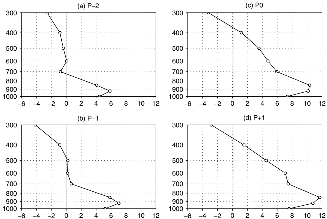
Figure 4. Nine-year composite vertical structure of U-wind in the box 70\text{--}85^\circ\text{E} and 5^\circ\text{--}10^\circ\text{N} for (a) P - 2 , (b) P - 1 , (c) P0 and (d) P + 1
