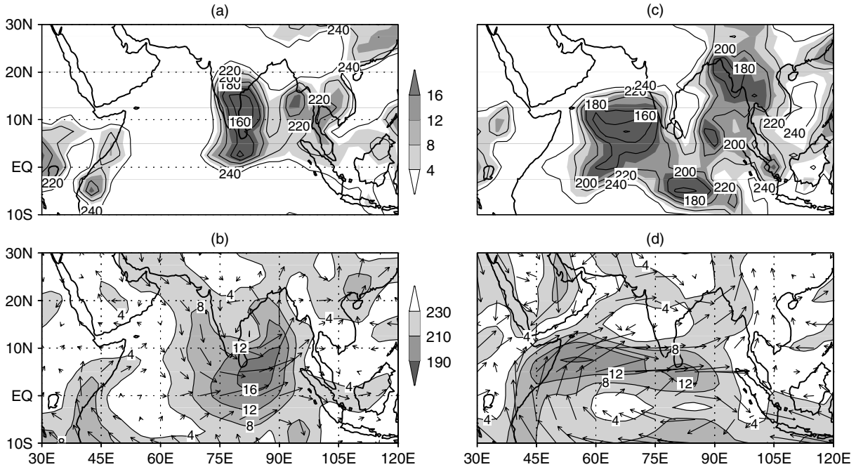
Figure 14. Pentad mean OLR for (a) 9–13 May 1979 and (c) 11–15 June, 1979. Contours less than 240 W/m 2 at intervals of 20 W/m 2 are shown in (a) and (c) and are shaded from 190 to 230 W/m 2 . Pentad mean 850 hPa wind (m/s) for (b) 9–13 May 1979 and for (d) 11–15 June 1979. Contours in (b) and (d) are drawn at intervals of 4 m/s and those above 4 m/s are shaded
