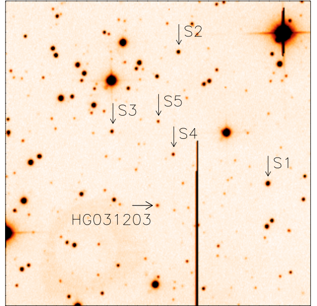
Fig. 1. I -band image of the field of HG 031203. North is up, east to the left; the image is 2' on a side. The positions of the host galaxy and of the comparison stars are noted. Blooming from a bright star, (outside this image) is visible as a N-S streak and a ring caused by reflection is evident just to the southeast of HG 031203.
