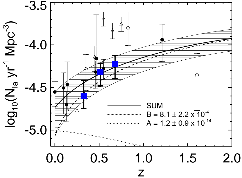
FIGURE 1. Observed SNLS SN Ia volumetric rate evolution. The filled squares are the SNLS rates in each of the three redshift bins. The filled circles are previously published SN Ia rates derived from samples primarily confirmed by spectroscopy from the following references (in redshift order): [5, 8, 10, 6, 9, 11, 7, 11]. The open circles are the SN Ia rates from [11] with samples having only 50% spectroscopic confirmation. The open triangles are the rates from [12], whose samples are confirmed almost entirely with photometric methods. Error bars represent the systematic and statistical errors added in quadrature.
