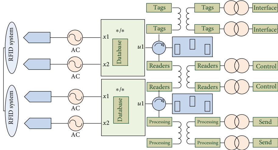
FIGURE 2: RFID system circuit composition.
