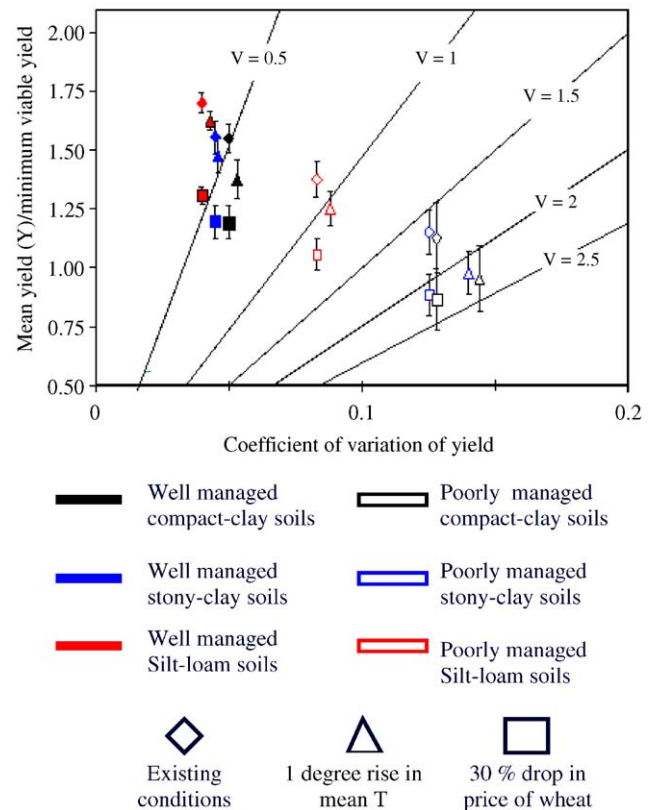
Fig. 3. Relative vulnerability of wheat yields to climate variability in the Yaqui Valley agricultural region. The lines are contours of equal relative vulnerability, where the values are normalized by the average farm unit (i.e. vulnerability of the average farm unit is one). Where color indicates soils type (red = silt loam, blue = stony clay, black-compact clay), solid shapes indicate good management and open shapes indicate poor management, the shape indicates differences among conditions (diamond = existing conditions, triangle = 1 degree rise in mean temperature, square = 30% drop in wheat price).
