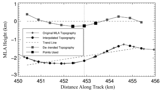
Figure 3. A schematic of how the spacing of MLA points is treated and the track detrended before calculation of \Delta h is performed (at L = 0.5 km). First, an MLA point of interest is selected (denoted by the vertical dotted line). Second, MLA points within 5 times the baseline of interest on either side of the point of interest (“Original MLA Topography”) are interpolated to produce spacing equivalent to the baseline of interest (“Interpolated Topography”). Third, a linear trend line is fit to the interpolated data (“Trend Line”) and used to remove broad-scale slopes, resulting in the De-trended Topography. Fourth, two \Delta h values are calculated for each point of interest using adjacent points (“Points Used”) to either side.
