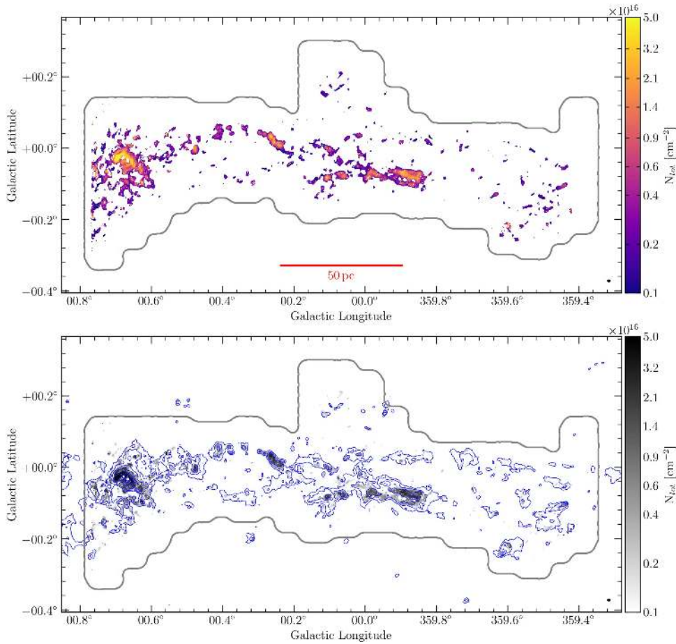
Figure 10. Top: total ammonia column density according to Equation (22). The dynamical range is \sim 5 \times 10^{15} \text{ cm}^{-2} to \sim 6.8 \times 10^{16} \text{ cm}^{-2} . In warm clouds like Sgr B2, this figure represents a lower limit as the unobserved states J > 6 can be populated in non-negligible fractions (Mills & Morris 2013). Bottom: the same map of the total column density overlaid with 870 \mu\text{m} dust emission from ATLASGAL (Schuller et al. 2009) at contours of powers of two (1, 2, ..., 64) \text{Jy beam}^{-1} . The ammonia distribution closely follows dust emission in regions of high ammonia column density ( \gtrsim 1 \times 10^{16} \text{ cm}^{-2} ).
