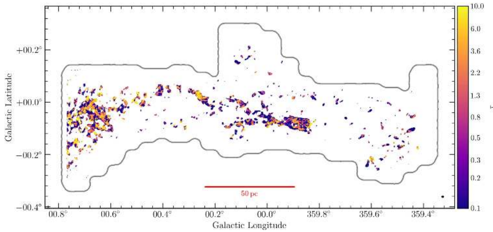
Figure 14. \text{NH}_3 (3, 3) opacity derived from fitting the hyperfine structure. Large areas in CMZ clouds are not optically thick ( \tau \lesssim 1 ) and either optically thin ( \tau \sim 0 ) or marginally thick ( \tau < 1 ). Several extreme exceptions of \tau \gtrsim 10 exist in the Brick, an extension to the 20 \text{ km s}^{-1} cloud, and the surrounding of Sgr B2.
