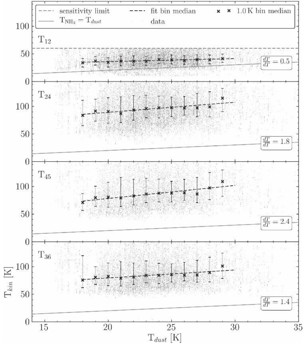
Figure 40. Correlation of the Hi-Gal dust temperature (Molinari et al. 2011) and the kinetic ammonia gas temperature as in Figure 17. The temperature estimate is labeled in the top left corner of each panel. Panels are zoomed to display the same range to allow a direct comparison.
