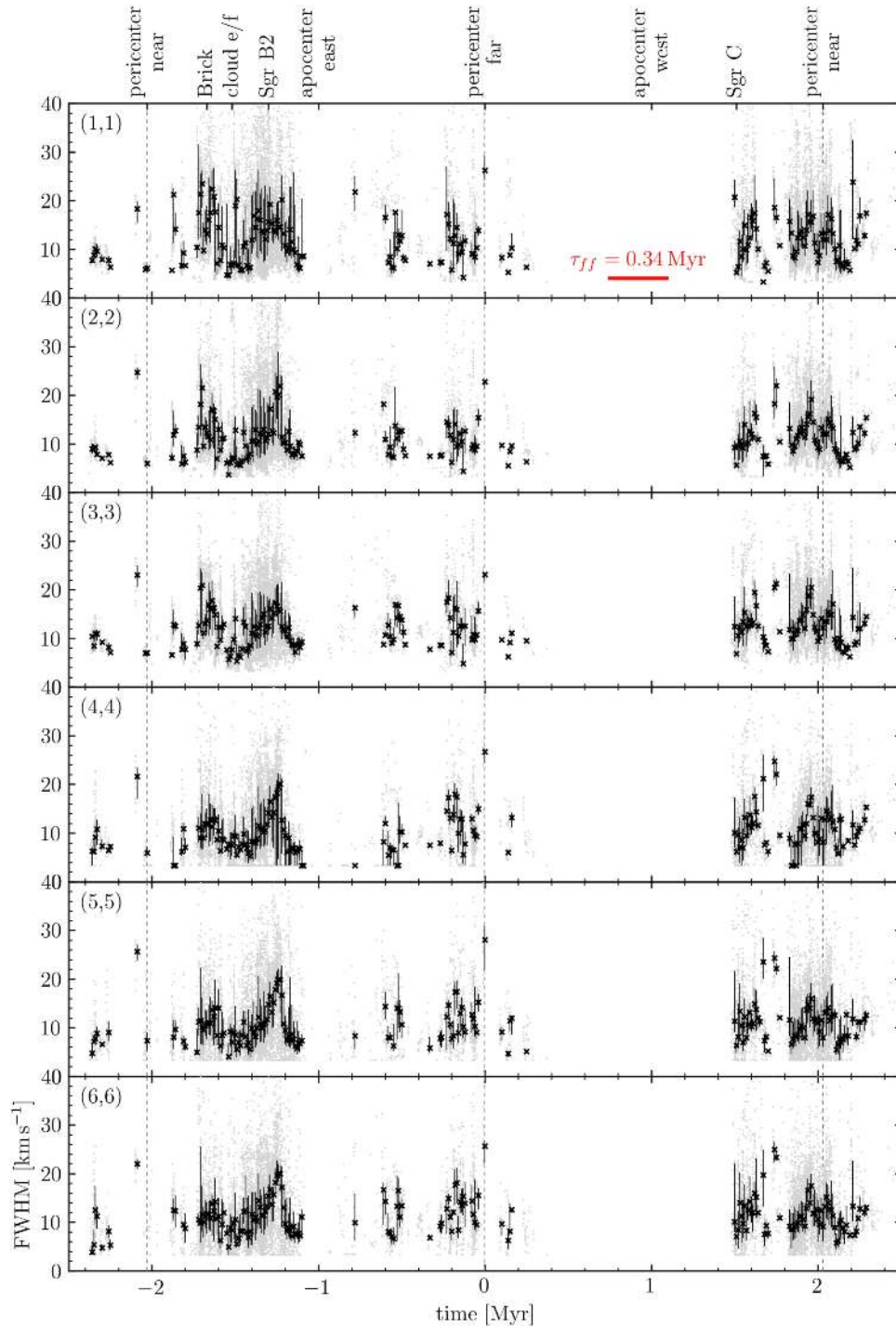
Figure 43. Ammonia line width as a function of time since far-side pericenter passage (bottom x -axis; the top x -axis shows important dynamical points in the K15 model and massive molecular clouds). The ammonia species is given in the top left corner of each panel. Vertical dashed lines highlight the occurrence of pericenter passages. Measurements for individual pixels (light gray points) are overlaid with black crosses denoting medians in bins of 0.01 Myr and error intervals that include 50% of the data in each bin.
