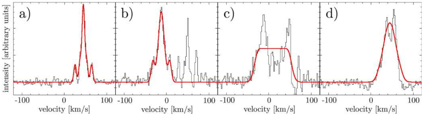
Figure 36. Examples of the ammonia hyperfine structure per pixel fits (red) to observed SWAG spectra (black). Satellite components blend with the main line because of the large line width (a), (b), and (c) or because of the blending of multiple lines along the line of sight (c) and (d). (a) Typical good fit of a single emission component along the line of sight. (b) For multiple components, the strongest component is usually fitted well. (c) Occasionally, two separated components of similar peak intensity may be fitted by an unphysically large line width. (d) When two (or more) components of similar intensity blend, they might be fitted as a single component with large line width. The latter two cases are excluded from further analyses by the large line width ((c), \sim 80 \text{ km s}^{-1} ) and bad fit quality as given by the reduced \chi^2 (d).
