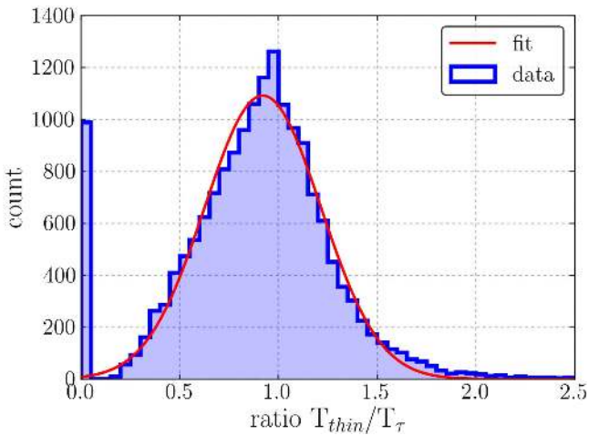
Figure 35. Histogram of the temperature ratio T_{\text{thin}}/T_{\tau} between the kinetic ammonia temperature T_{24} derived assuming optically thin emission and considering measured opacities (Figure 34). For \sim 1000 pixels at a ratio of 0.0, the hyperfine structure could be fitted and an opacity-corrected temperature derived, although the emission is faint enough to be masked while calculating the image moment 0 on which the temperature under thin assumption is based. The inverse case (ratios of +\infty ) occurs more often, but does not show up in this plot. A Gaussian fit generally describes the distribution well, but does not fit a greater amount of temperature ratios of 1.0 and 1.5–2.0. The latter is the effect of considering the opacity for optically thick emission. As lower ammonia states are typically more occupied (falling slope in Boltzmann plot) and the opacity correction increases occupation over the thin approximation ( N_{\tau} > N_{\text{thin}} ), the temperature decreases ( T_{\tau} < T_{\text{thin}} ) and thus T_{\text{thin}}/T_{\tau} > 1.0 .
