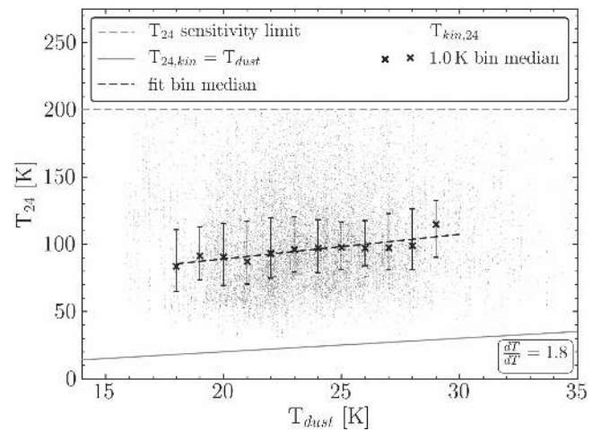
Figure 17. Correlation of Hi-Gal dust temperature (Molinari et al. 2011) and kinetic ammonia gas temperature T_{24} . Black crosses denote median T_{24} temperature in bins of 1.0 K dust temperature, which are linearly fitted (black dashed line). The errors are the range that includes 50% of measurements in the respective bin. Median temperatures are correlated despite the offset relative to T_{24} = T_{\text{dust}} .
