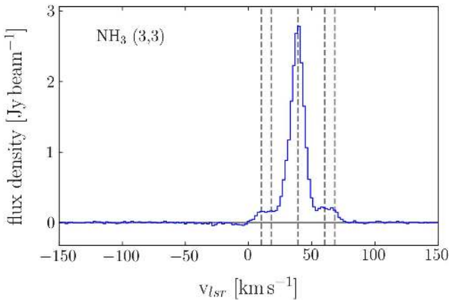
Figure 6. Sample spectrum toward the Brick ( l = 0^\circ 2328 , b = 0^\circ 0107 ) extracted from the \text{NH}_3 (3, 3) cube. rms noise is 13.1 \text{ mJy beam}^{-1} (0.061 K). The positions of the hyperfine satellites according to Table 3 are indicated by dashed vertical lines. Note the broad line width that blends the outer hyperfine components (which have separations of \pm 21.1 \text{ km s}^{-1} and \pm 29.1 \text{ km s}^{-1} from the main line) into a pedestal.
