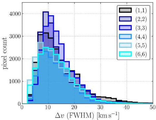
Figure 13. Distribution of FWHM of metastable ammonia hyperfine lines in the GC. The bin size of 2 \text{ km s}^{-1} corresponds to the spectral resolution of the data cubes.
