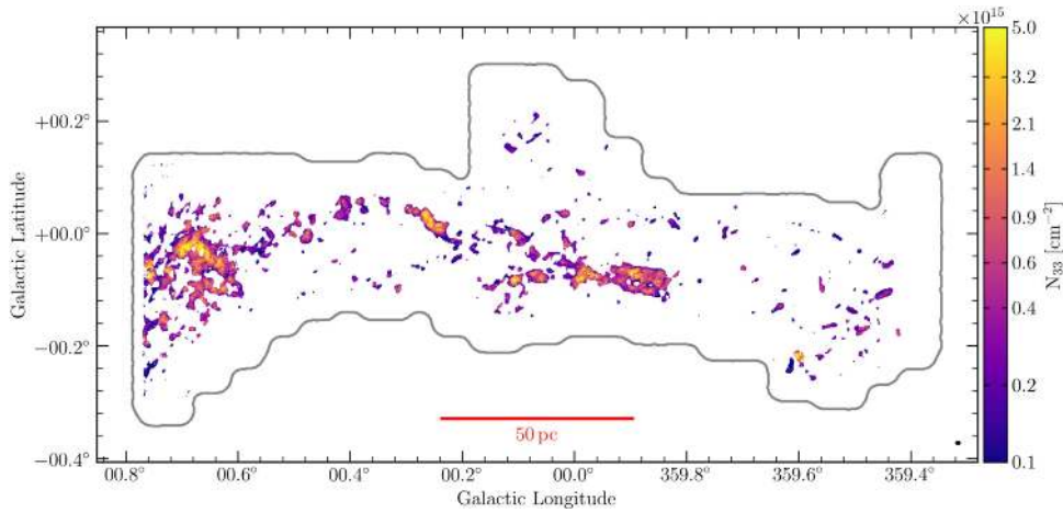
Figure 33. \text{NH}_3 (3, 3) column density N_l under consideration of non-zero opacity as derived by Equation (18) from fitting the hyperfine structure.
