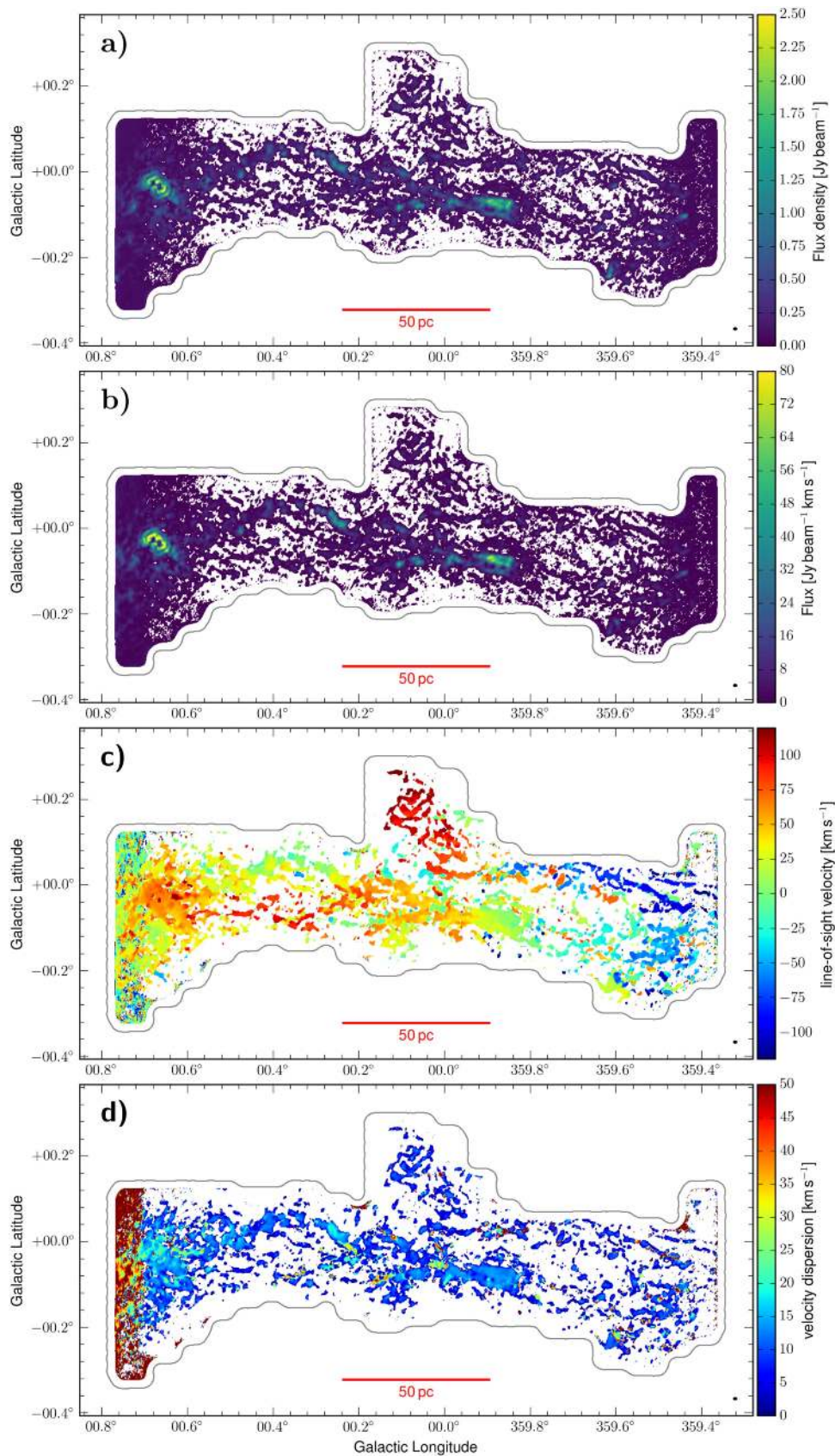
Figure 28. NH 3 (1, 1) moment maps: (a) peak intensity, (b) integrated intensity (moment 0), (c) intensity-weighted mean velocity (moment 1), and (d) intensity-weighted velocity dispersion (moment 2). The intensity maps (a) and (b) are masked at 3\sigma , velocity maps (c) and (d) are masked at 5\sigma with an rms noise of \sigma = 13.4 mJy. The beam of 26''.2 \times 17''.8 ( 1.06 pc \times 0.72 pc) is indicated in the lower right corner of each panel.
