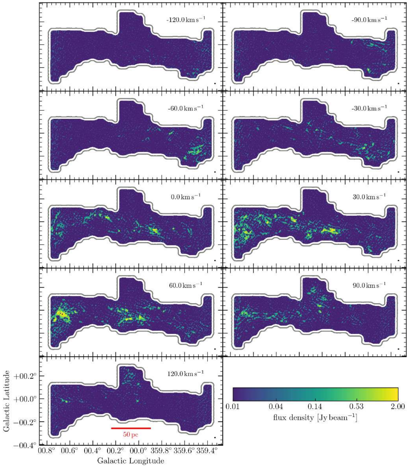
Figure 5. Channel maps of \text{NH}_3 (3, 3). Every fifteenth channel of 2 \text{ km s}^{-1} (separated by 30 \text{ km s}^{-1} ) in the range of -120 \text{ km s}^{-1} to +120 \text{ km s}^{-1} is shown. Velocity and beam ( 26''03 \times 17''71 , 89^\circ 3 ) are indicated in the top and bottom right corners, respectively. The conversion factor from flux density to brightness temperature for this beam size at 23.87 \text{ GHz} is T [\text{K}]/S [\text{Jy beam}^{-1}] = 4.65 .
