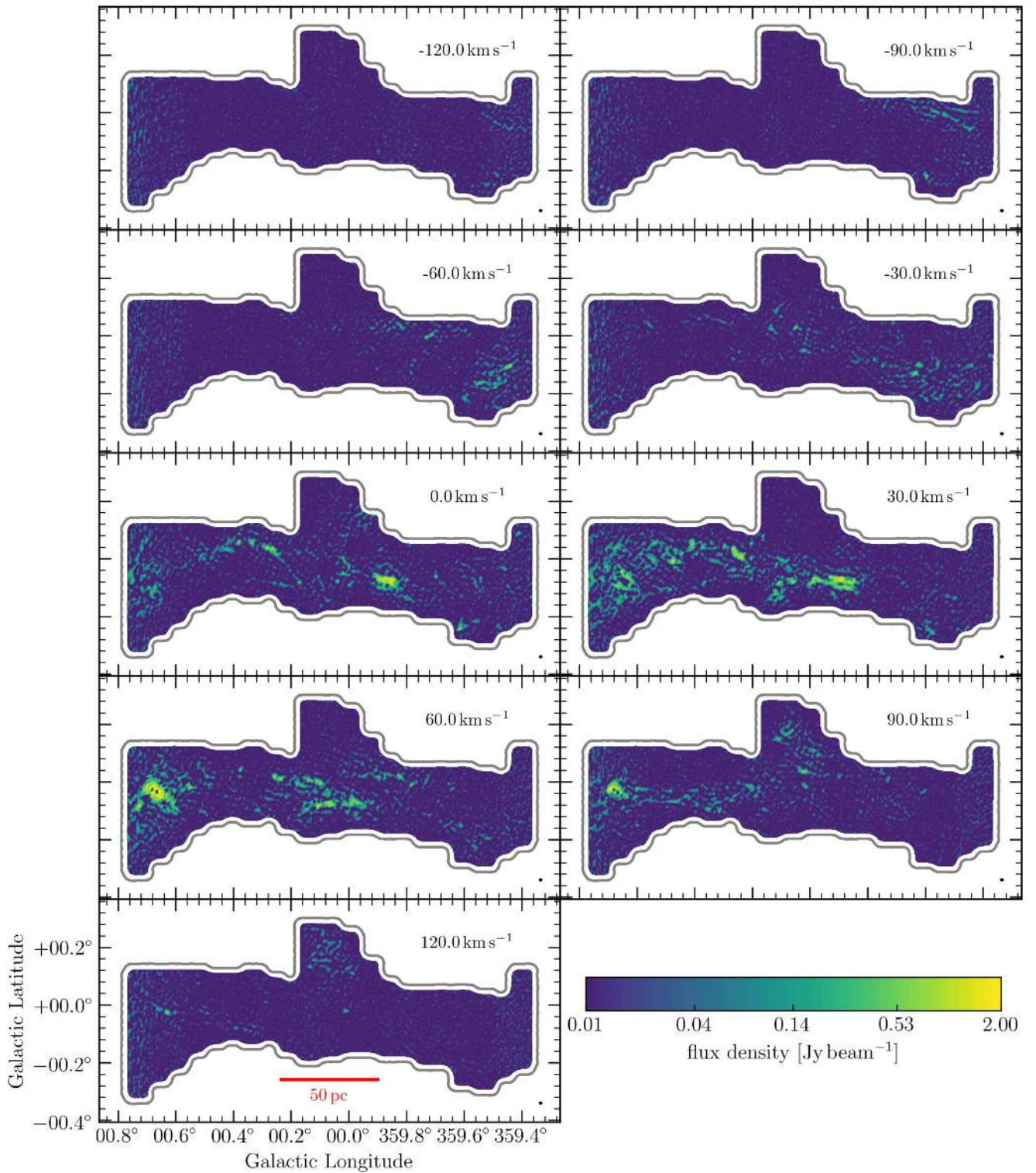
Figure 22. Channel maps of \text{NH}_3 (1, 1). Every fifteenth channel of 2 \text{ km s}^{-1} (separated by 30 \text{ km s}^{-1} ) in the range of -120 \text{ km s}^{-1} to +120 \text{ km s}^{-1} is shown. Velocity and beam area ( 26''22 \times 17''84 , 89^\circ3 ) are indicated in the top and bottom left corners, respectively. The conversion factor from flux density in \text{Jy beam}^{-1} to brightness temperature in K for this beam size at 23.69 \text{ GHz} is T [\text{K}]/S [\text{Jy beam}^{-1}] = 4.65 .
