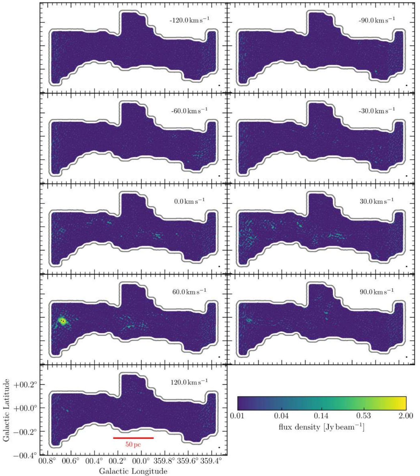
Figure 25. Channel maps of \text{NH}_3 (5, 5). Every fifteenth channel of 2 \text{ km s}^{-1} (separated by 30 \text{ km s}^{-1} ) in the range of -120 \text{ km s}^{-1} to +120 \text{ km s}^{-1} is shown. Velocity and beam ( 25''32 \times 17''23 , 89^\circ3 ) are indicated in the top and bottom left corners, respectively. The conversion factor from flux density in \text{Jy beam}^{-1} to brightness temperature in K for this beam size at 24.53 \text{ GHz} is T [\text{K}]/S [\text{Jy beam}^{-1}] = 4.65 .
