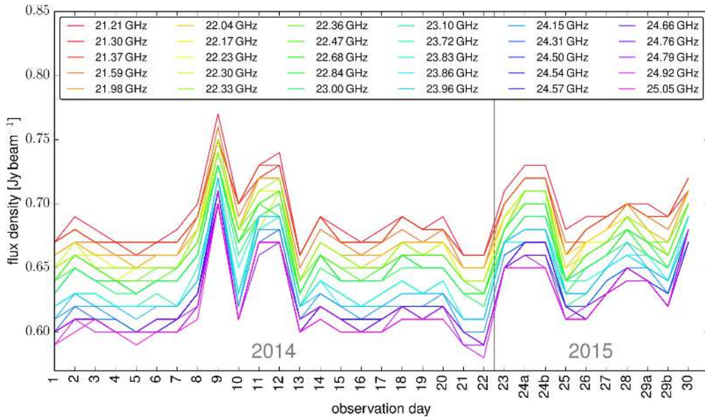
Figure 4. Flux density of the phase calibrator PKS 1710-269 per observation day after all calibration steps for the 30 frequency bands of CABB. On observation days 24 and 29, correlator crashes required new calibrations, which are labeled a and b and correspond to flux densities before and after the crash, respectively. Flux densities are constant across observation days within \sim 15\% . The increasing values toward lower frequency is an intrinsic property of the source: a quasar with spectral index \sim -0.5 . The precision of the MIRIAD task imstat is two decimal places, which leads to quantized data.
