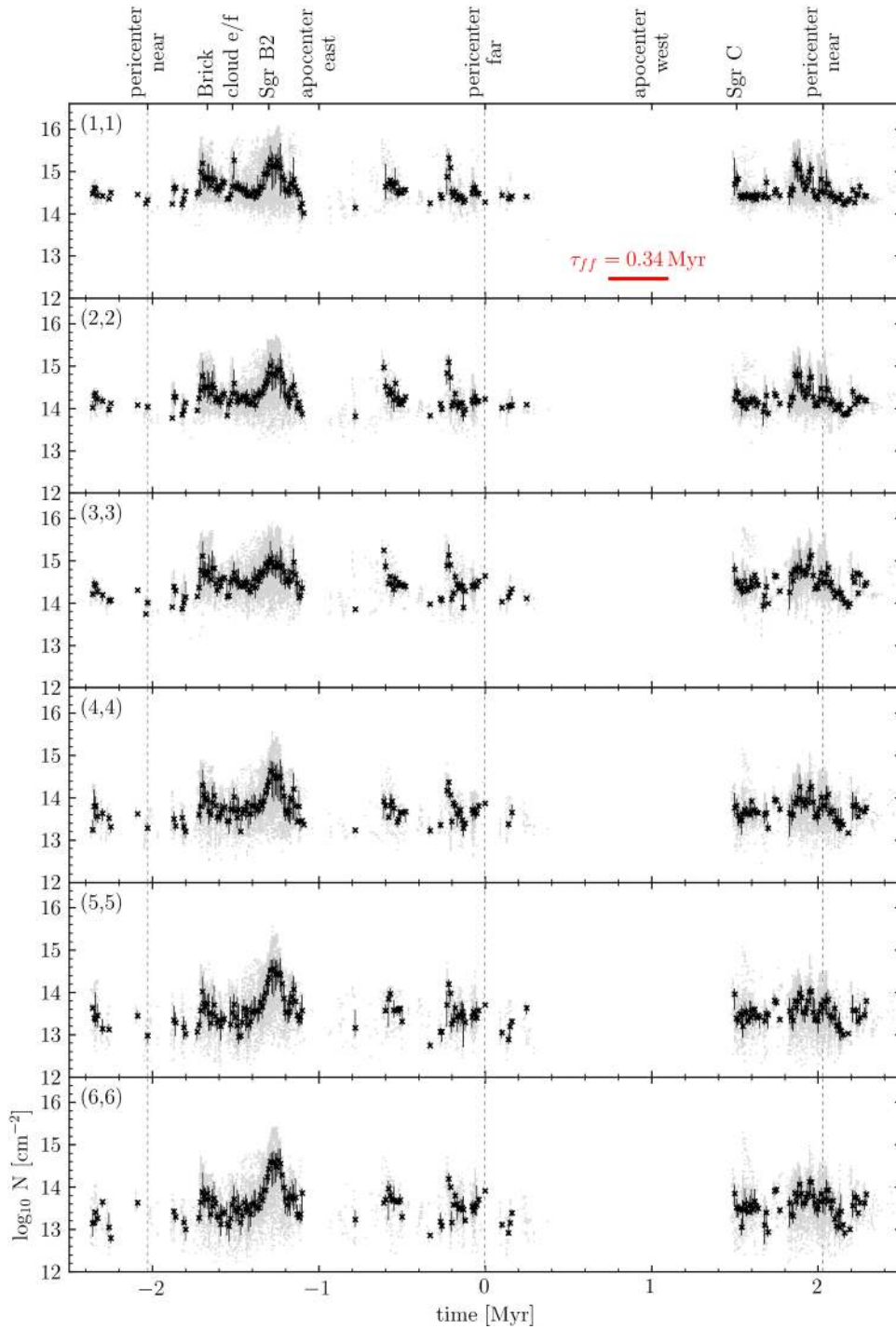
Figure 42. Ammonia column density as a function of time since far-side pericenter passage (bottom x -axis; the top x -axis shows important dynamical points in the K15 model and massive molecular clouds). The ammonia species is given in the top left corner of each panel. Vertical dashed lines highlight the occurrence of pericenter passages. Measurements for individual pixels (light gray points) are overlaid with black crosses denoting medians in bins of 0.01 Myr and error intervals that include 50% of the data in each bin.
