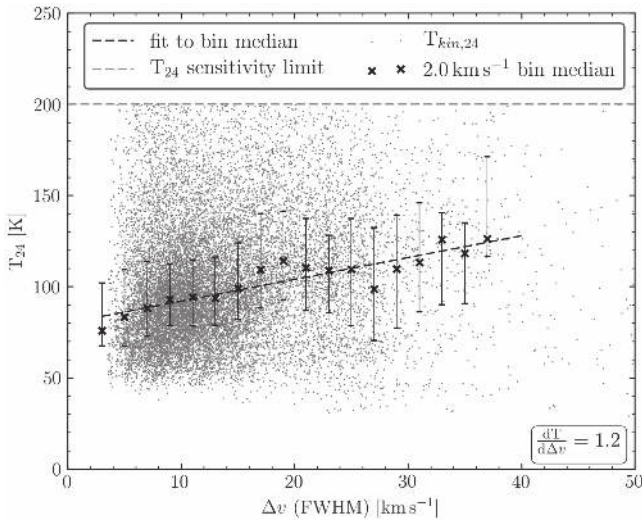
Figure 18. Kinetic ammonia temperature T_{24} as a function of line width of \text{NH}_3 (2, 2). Median temperatures in bins of 2.0 \text{ km s}^{-1} width are marked by black crosses and fitted linearly. The errors are the range that includes 50% of measurements in the respective bin. A cutoff at 200 K is applied, above which the conversion of rotational into kinetic temperature becomes increasingly unreliable (Table 4, Morris et al. 1973; Ott et al. 2011; Gorski et al. 2017).
