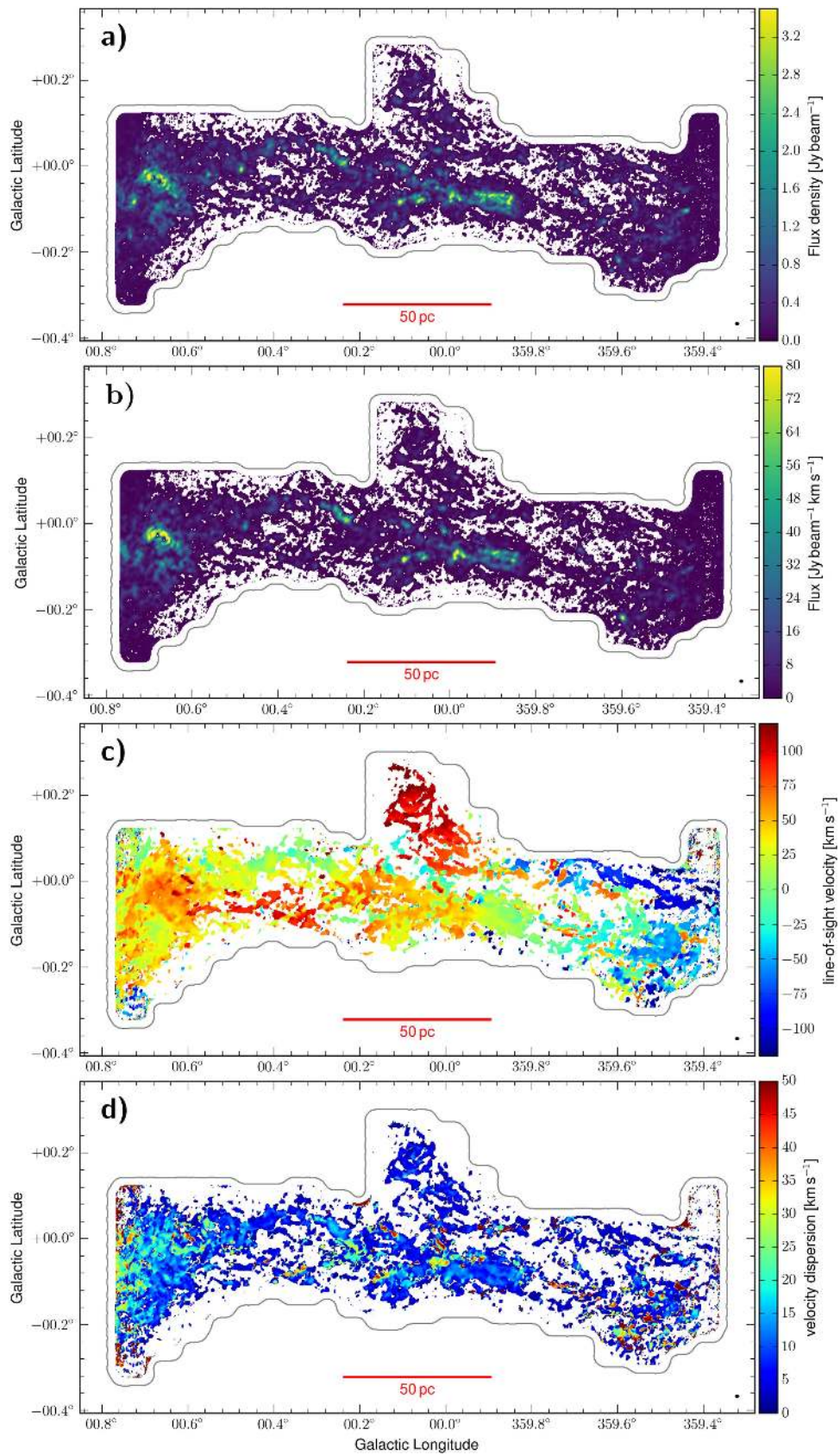
Figure 7. \text{NH}_3 (3, 3) moment maps: (a) peak intensity, (b) integrated intensity (moment 0), (c) intensity-weighted mean velocity (moment 1), and (d) intensity-weighted velocity dispersion (moment 2). The intensity maps (a) and (b) are masked at 3\sigma , and velocity maps (c) and (d) are masked at 5\sigma with an rms noise of \sigma = 13.1 mJy. The beam of 26''0 \times 17''7 ( 1.05 pc \times 0.71 pc) is indicated in the lower right-hand corner of each panel.
