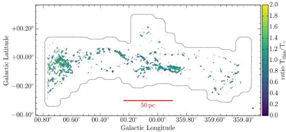
Figure 34. Ratio map T_{\text{thin}}/T_{\tau} of the ammonia T_{24} temperature assuming optically thin emission ( T_{\text{thin}} ) and considering opacity effects ( T_{\tau} ). The differences are minor (blue-green) in large areas of the map, but the temperature can be overestimated (yellow) in dense regions by factors of \sim 2.0 . Temperatures in less dense clouds and at the edges of the fitted area are underestimated (dark blue).
