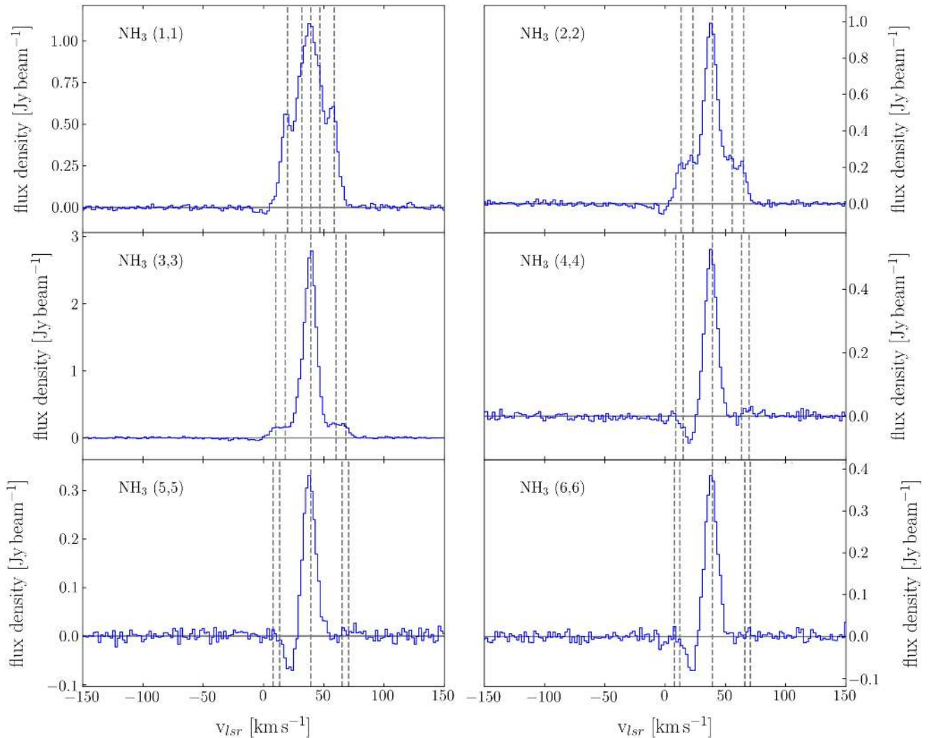
Figure 27. Example spectra with independent scaling of the y-axis toward the Brick extracted from the \text{NH}_3 (1, 1) to (6,6) data cubes. The rms noise is 0.062 K, 0.061 K, 0.061 K, 0.060 K, 0.056 K, and 0.061 K, respectively. The positions of the hyperfine satellites according to Table 3 are indicated by dashed vertical lines. Note the complex structure of broad line widths blending hyperfine components and an absorption component at \sim 20 \text{ km s}^{-1} in the higher lines.
