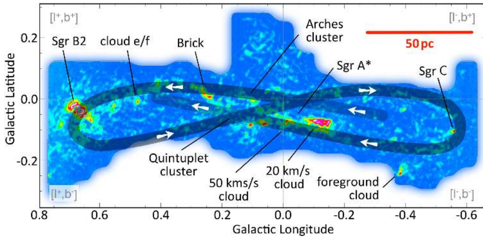
Figure 1. Overview of the GC. The gas (background, SWAG \text{NH}_3 (3, 3) peak intensity) resembles the shape of an infinity symbol, \infty , and is parametrized as a sequence of stream segments by K15. The direction of motion is along the dust ridge ( [l^+, b^+] denoting positive longitude and latitude) to Sgr B2, [l^+, b^-] , [l^-, b^+] to Sgr C and [l^-, b^-] . Gas in the dust ridge [l^+, b^+] and [l^-, b^-] is mostly on the near side (in front of the GC), whereas [l^+, b^-] and [l^-, b^+] gas is mostly on the far side (Bally et al. 2010; Molinari et al. 2011). The most important sources are labeled.
