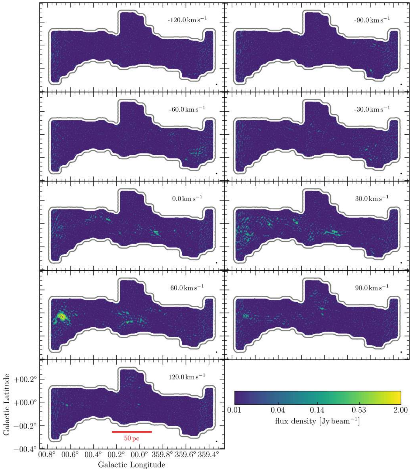
Figure 24. Channel maps of \text{NH}_3 (4, 4). Every fifteenth channel of 2 \text{ km s}^{-1} (separated by 30 \text{ km s}^{-1} ) in the range of -120 \text{ km s}^{-1} to +120 \text{ km s}^{-1} is shown. Velocity and beam ( 25''74 \times 17''51 , 89^\circ:3 ) are indicated in the top and bottom left corners, respectively. The conversion factor from flux density in \text{Jy beam}^{-1} to brightness temperature in K for this beam size at 24.14 \text{ GHz} is T [\text{K}]/S [\text{Jy beam}^{-1}] = 4.65 .
