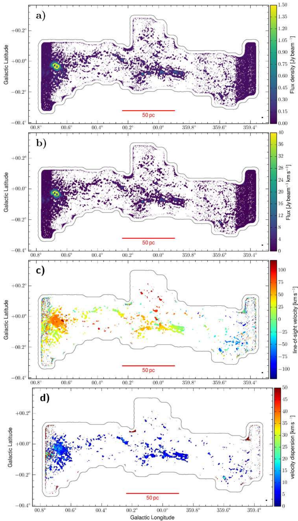
Figure 32. \text{NH}_3 (6, 6) moment maps: (a) peak intensity, (b) integrated intensity (moment 0), (c) intensity-weighted mean velocity (moment 1), and (d) intensity-weighted velocity dispersion (moment 2). The intensity maps (a) and (b) are masked at 3\sigma , velocity maps (c) and (d) are masked at 5\sigma with an rms noise of \sigma = 13.2 mJy. The beam of 24''.8 \times 16''.9 ( 1.00 \text{ pc} \times 0.68 \text{ pc} ) is indicated in the lower right corner of each panel.
