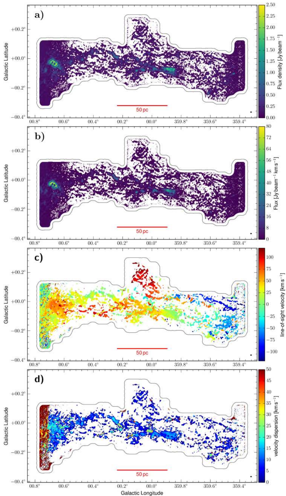
Figure 29. \text{NH}_3 (2, 2) moment maps: (a) peak intensity, (b) integrated intensity (moment 0), (c) intensity-weighted mean velocity (moment 1), and (d) intensity-weighted velocity dispersion (moment 2). The intensity maps (a) and (b) are masked at 3\sigma , velocity maps (c) and (d) are masked at 5\sigma with an rms noise of \sigma = 13.1 mJy. The beam of 26.2 \times 17''.8 ( 1.05 \text{ pc} \times 0.72 \text{ pc} ) is indicated in the lower right corner of each panel.
