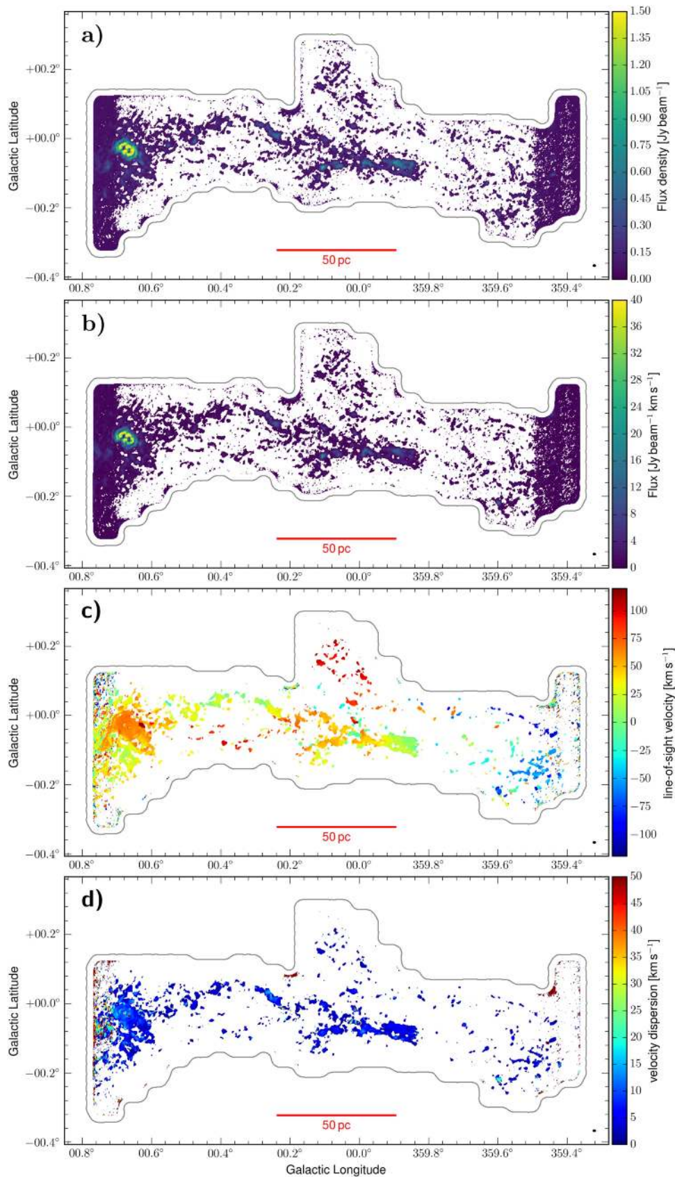
Figure 30. \text{NH}_3 (4, 4) moment maps: (a) peak intensity, (b) integrated intensity (moment 0), (c) intensity-weighted mean velocity (moment 1), and (d) intensity-weighted velocity dispersion (moment 2). The intensity maps (a) and (b) are masked at 3\sigma , velocity maps (c) and (d) are masked at 5\sigma with an rms noise of \sigma = 12.9 mJy. The beam of 25''.7 \times 17''.5 ( 1.04 \text{ pc} \times 0.70 \text{ pc} ) is indicated in the lower right corner of each panel.
