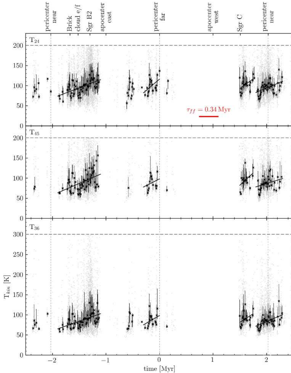
Figure 41. Kinetic ammonia temperature as a function of time since far-side pericenter passage (bottom x -axis; the top x -axis shows important dynamical points in the K15 model and massive molecular clouds). The temperature tracer is given in the top left corner of each panel. A horizontal dashed gray line denotes the sensitivity limit of the conversion from rotational into kinetic temperature. Vertical dashed lines highlight the occurrence of pericenter passages. Measurements for individual pixels (light gray points) are overlaid with black crosses denoting medians in bins of 0.01 Myr and error intervals that include 50% of the data in each bin.
