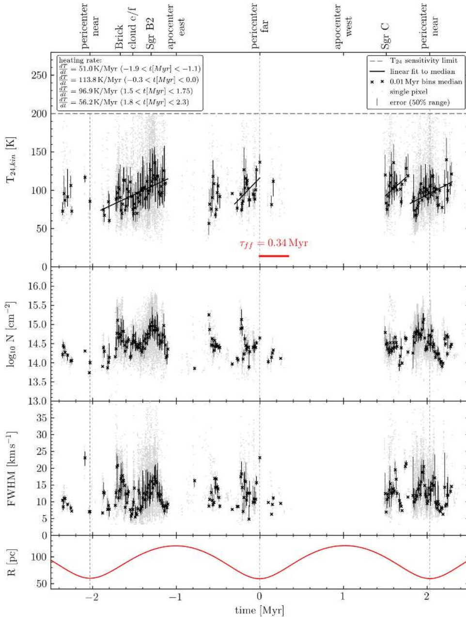
Figure 20. Kinetic ammonia temperature T_{24} (top), \text{NH}_3 (3, 3) column density (middle top), and \text{NH}_3 (3, 3) line width (middle bottom) as a function of time since far-side pericenter passage (bottom x-axis, top x-axis shows important dynamical points in the K15 model and massive molecular clouds). The bottom panel shows the radial distance from the center of the Galactic potential. Measurements for individual pixels (light gray points) are overlaid with black crosses denoting medians in bins of 0.01 Myr and error intervals that include 50% of the data in each bin. Linear fits to the median temperature and corresponding heating rates are shown for four regions of consistent time evolution.
