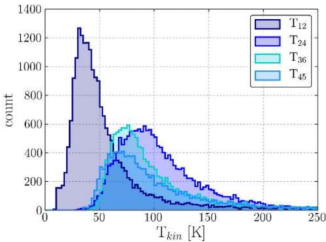
Figure 16. Distribution of temperatures in the GC as derived for four kinetic ammonia gas temperatures. The conversion of rotational to kinetic temperature is taken from Ott et al. (2011), as described in Section C. T_{ij} denotes the temperature measure derived from the lines \text{NH}_3 (i, i) and \text{NH}_3 (j, j). T_{12} is sensitive to cold gas, whereas higher lines need warmer conditions to be excited and are thus susceptible only to increasingly warm gas. T_{24} , T_{45} , and T_{36} trace similarly warm gas of >50 K.
