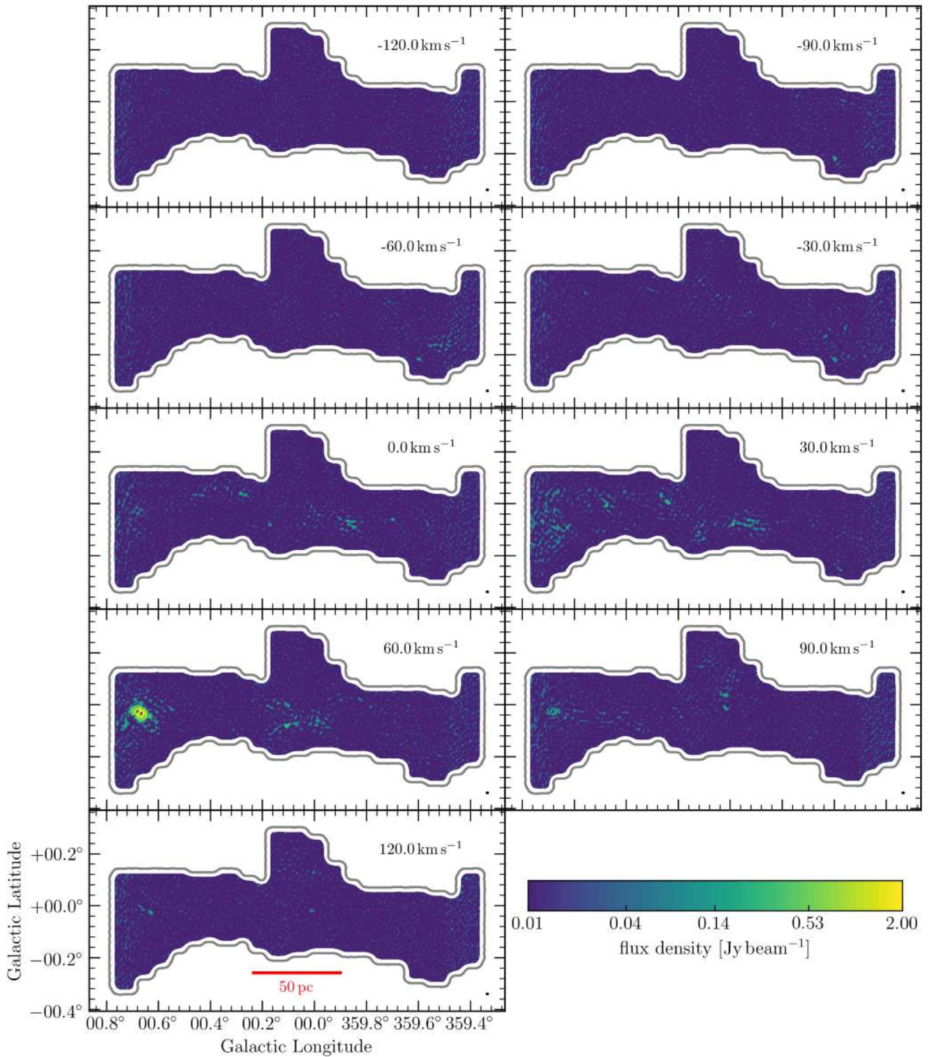
Figure 26. Channel maps of \text{NH}_3 (6, 6). Every fifteenth channel of 2 \text{ km s}^{-1} (separated by 30 \text{ km s}^{-1} ) in the range of -120 \text{ km s}^{-1} to +120 \text{ km s}^{-1} is shown. Velocity and beam ( 24''80 \times 16''87 , 89^\circ3 ) are indicated in the top and bottom left corners, respectively. The conversion factor from flux density in \text{Jy beam}^{-1} to brightness temperature in K for this beam size at 25.06 \text{ GHz} is T [\text{K}]/S [\text{Jy beam}^{-1}] = 4.65 .
