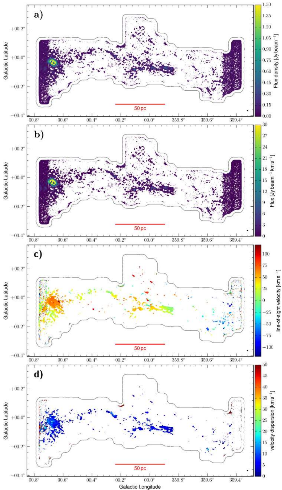
Figure 31. \text{NH}_3 (5, 5) moment maps: (a) peak intensity, (b) integrated intensity (moment 0), (c) intensity-weighted mean velocity (moment 1), and (d) intensity-weighted velocity dispersion (moment 2). The intensity maps (a) and (b) are masked at 3\sigma , velocity maps (c) and (d) are masked at 5\sigma with an rms noise of \sigma = 12.0 mJy. The beam of 25'' \times 17'' ( 1.02 \text{ pc} \times 0.69 \text{ pc} ) is indicated in the lower right corner of each panel.
