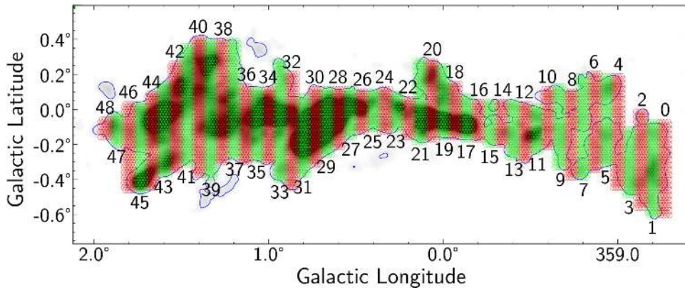
Figure 2. SWAG observing layout. The spatial coverage of SWAG is derived from the 0.1 \text{ K km s}^{-1} contour (blue) of the Mopra single-dish CMZ survey by Ott et al. (2014; background gray-scale image). Between 40 to 220 pointings are included in an observation strip (numbered from west to east and alternately colored). This work includes data of the inner CMZ covered by strips 10 to 30.
