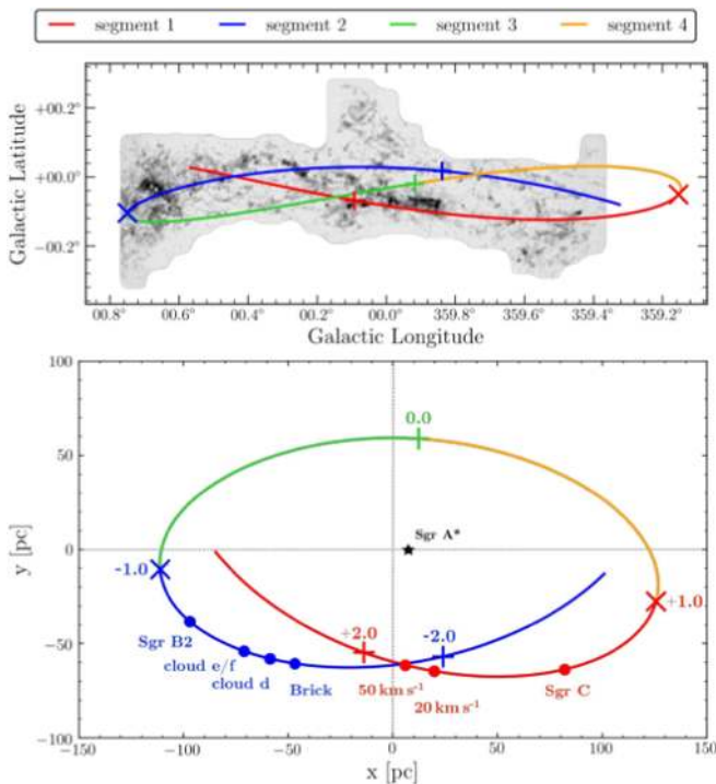
Figure 19. Overview of the stream orbit according to K15. Pericenters are marked by plus symbols, crosses denote apocenters. The bottom of the gravitational potential at Sgr A* is marked by a star. Top: projected view of the stream orbit in Galactic coordinates. Background image: SWAG \text{NH}_3 (3, 3) integrated intensity. Bottom: top-down view in physical coordinates. The observer is situated in negative y -direction. Major molecular clouds are labeled. Time since far-side pericenter passage is given for peri- and apocenters in Myr.
