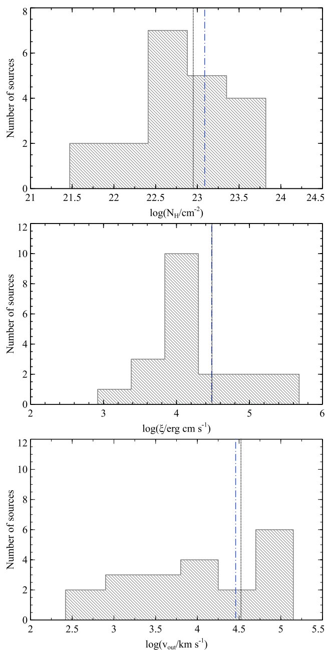
Figure 8. Histogram showing the overall distributions of mean absorber parameters for each source: (a) logarithm of the mean column density; (b) logarithm of the mean ionization parameter; (c) logarithm of the mean outflow velocity. The dot-dashed (blue) and dotted (black) vertical lines indicate the mean value of the Suzaku and XMM-Newton analyses, respectively.
