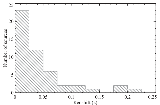
Figure 1. Histogram showing the distribution of sources included in this work. The high red-shift QSO APM 08279+5255 ( z = 3.91 ) has been omitted for scaling purposes.
