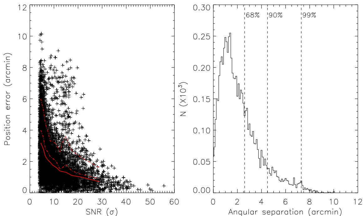
Fig. 3.— Left: Scatter plot of position error versus source detection significance. We have parameterized the distribution and show in the red curves (from bottom to top): the best fit to the distribution (solid), the 68% confidence limit (C.L.), and the 90% C.L. Right: Histogram of angular separations between the BAT position and the best catalog position (averaged over all values of SNR). Source positions have an accuracy of less than what is indicated by the vertical lines in, from left to right, 68%, 90% or 95% of cases.
