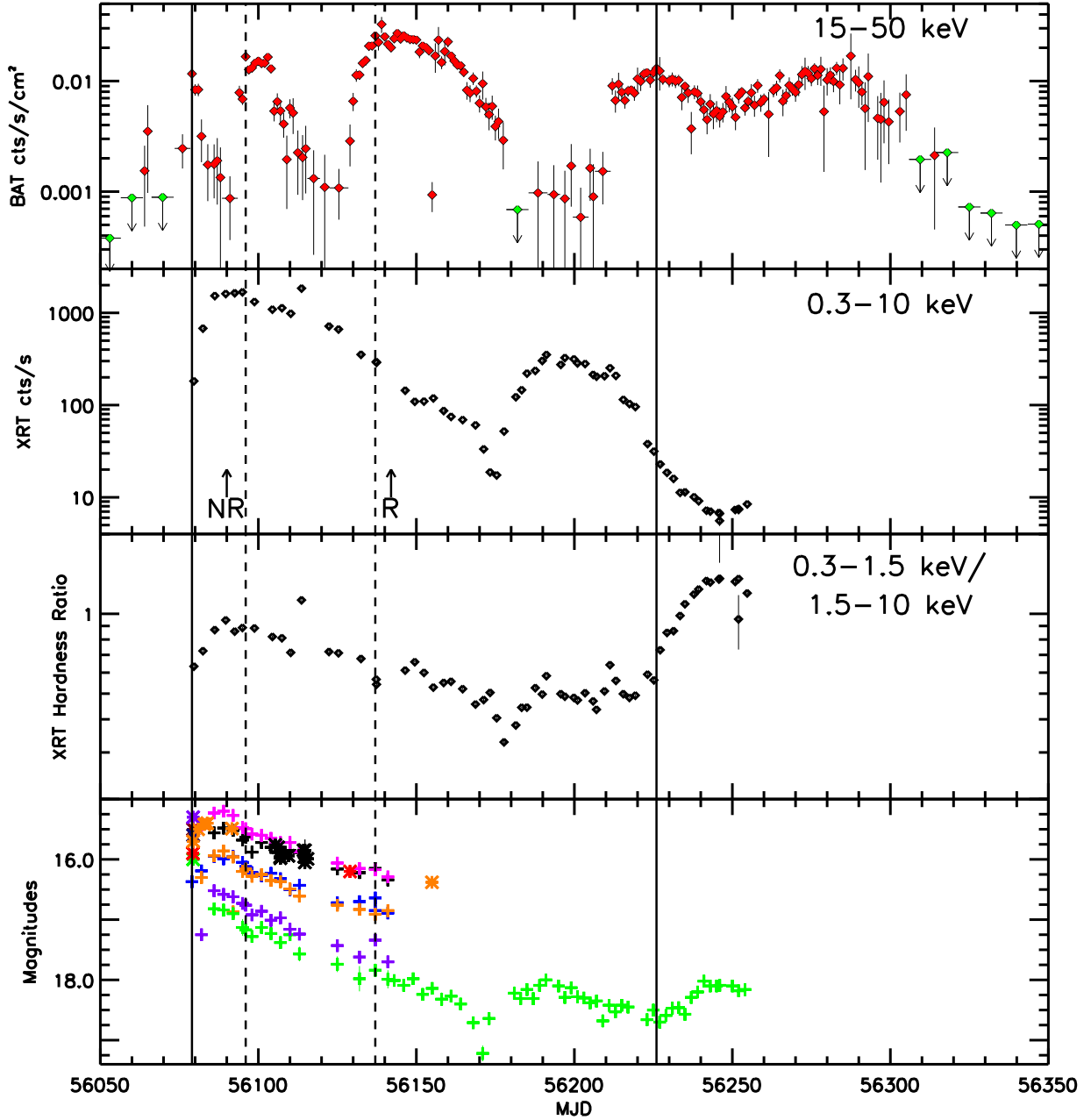
Fig. 17.— Light curves for Swift J1910.2–0546 from BAT (upper panel), XRT (second panel) and optical observations (lower panel) and XRT hardness ratio (third panel). The dashed vertical lines indicate the approximate dates of the peaks in the BAT light curve. The dashed lines represent the times of the two BAT on-board triggers on this source. Swift was unable to observe Swift J1910.2–0546 with the NFIs between MJD 56254 and 56360 due to the Sun observing constraint. In the bottom plot crosses represent Swift/UVOT filters: black = v, blue = b, magenta = u, orange = uvw1, green = uvm2, purple = uvw2. The stars indicate the following filters: black = V, red = R, orange = r', green = g', purple = z', blue = K, brick red = H. The red stars are from Cenko & Ofek (2012, MJD 56079) and Casares et al. (2012, MJD 56129). The black stars are from Lloyd et al. (2012) and the orange stars are from Rau, Greiner & Schady (2012, MJD 56079), Britt, Johnson & Hynes (2012, MJD 56080 - 56083), Lloyd et al. (2012, MJD 56092), and Casares et al. (2012, MJD 56155). All other stars are from GROND (Rau, Greiner & Schady 2012). The arrows on the second panel indicate the times of a radio non-detection (NR, Fogasy, Yang & Paragi 2012) and radio detection (R, King et al. 2012)
