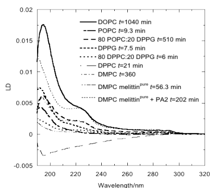
Figure Maximum LD spectra obtained for melittin PA2 (0.1 mg/mL) added to liposomes at lipid:peptide ratio of 100:1. Times and lipids are indicated on the figure.
