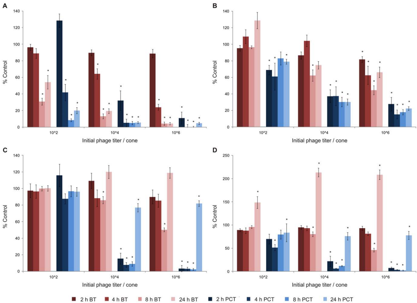
Figure 2. Phage \phi 15-mediated biofilm degradation. 24 h (A) and 48 h (B) old biofilm of PpG1. 24 h (C) and 48 h (D) old biofilm of RD5PR2. Biofilms grown on cones for 24 or 48 h, were initially inoculated with 10^2 , 10^4 and 10^6 pfu of phage \phi 15. After 2, 4, 8 and 24 h of phage treatment at 30°C, mean biofilm (BT: biofilm treatment) and planktonic survival (PCT: planktonic culture treatment) for n=20 cones or corresponding microtiter plate wells, respectively, were scored relative to untreated control samples (100%) and represented on the Y-axes. Five independent experiments were performed, each starting from a different overnight culture and each with four repeats for each parameter combination giving rise to an overall twentyfold repetition. Error bars indicate SEM. Significant values (two-tailed t test; P < 0.01 ) are marked by an asterisk (*). doi:10.1371/journal.pone.0018597.g002
