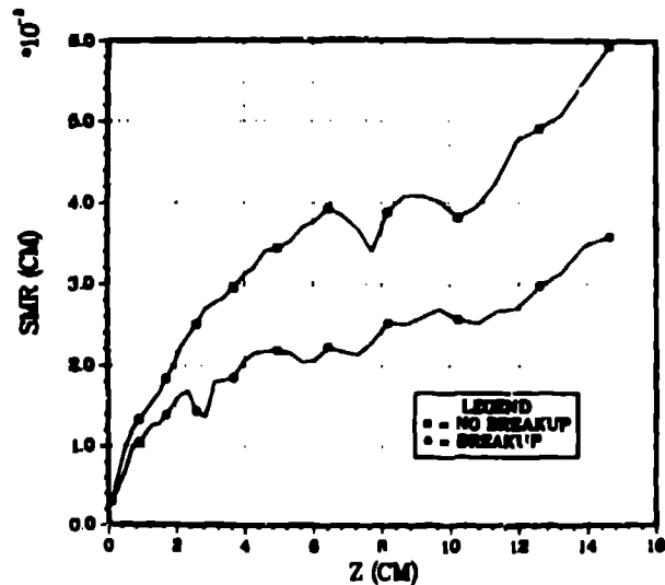
Fig. 7. Computed Sauter mean radii in calculations with and without breakup.
