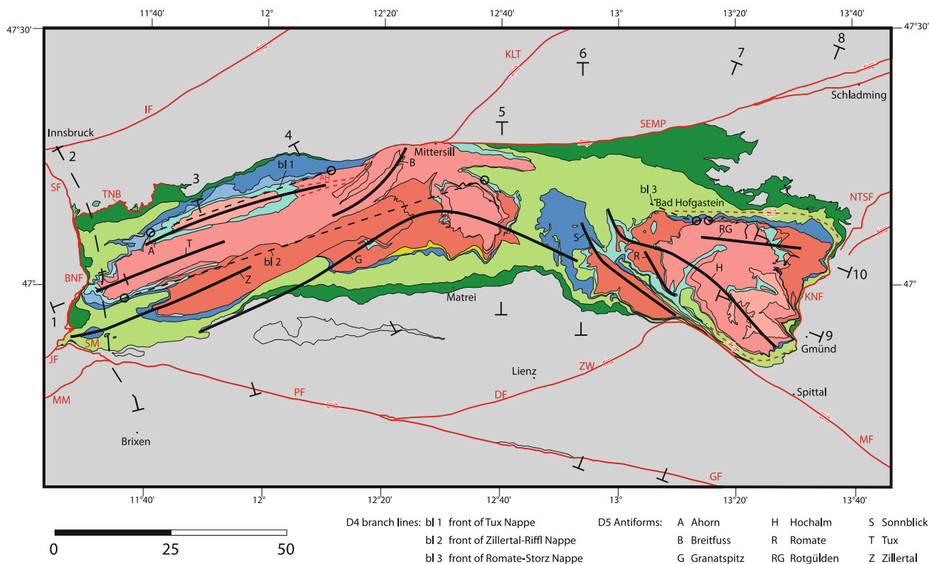
Fig. 4 Simplified tectonic map of the Tauern Window focussed on the internal structure of the Subpenninic and Penninic units. The hinge lines of the post-duplex (D5) antiforms are shown a thick black lines and selected branch lines related to duplex formation (D4) are shown as dashed black lines . Also shown are the traces of the cross-
