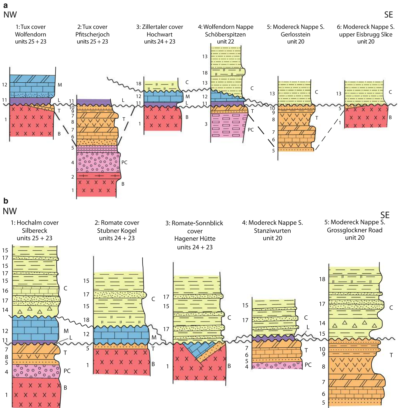
Fig. 2 Lithostratigraphic columns of the late Palaeozoic and Mesozoic cover of the Subpenninic nappes. a Western Tauern Window, b Eastern Tauern Window. The columns within the individual Fig. 2a, b are arranged according to the inferred palaeogeographical position going from NW (left) to SE (right). The stratigraphical logs were largely compiled from data by Alber (1976), Brandner et al. (2008), Exner (1982), Frisch (1975, 1980b), Frasl and Frank (1966), Höfer and Tichy (2005), Klebelsberg (1940), Kurz (2006), Kurz et al. (1998), Lammerer (1986), Lemoine (2003), Rockenschaub et al. (2003a), Thiele (1970), Veselá and Lammerer (2008), Veselá et al. (2008). Partly they are based on own observations. The lithologies are indicated with numbers, as follows: 1 granite gneiss; 2 Variscan
