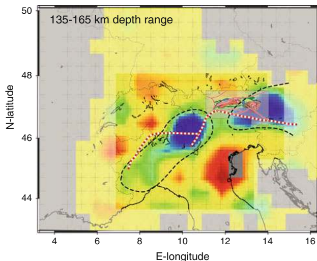
Fig. 5 Horizontal depth section at ca. 150 km depth (data from 135–165 km) through the 3-D V_p model of Lippitsch et al. (2003, their Fig. 13) superimposed with the outlines of the Tauern Window (see Fig. 1) and the trace of the Periadriatic Fault, offset by the Giudicarie Line (red stippled line). The depth section illustrates the variations in V_p within the upper mantle relative to the chosen 1D initial model. The positive velocity anomalies of >4\% V_p (dark blue) are interpreted as a SE-dipping European lithosphere in the Western Alps and a NE-dipping Adriatic lithosphere in the Eastern Alps (see Lippitsch et al. 2003 and Kissling et al. 2006 for further details). Note that the transition zone between the two high-velocity anomalies is located beneath the Giudicarie Line and the western part of the Tauern Window
