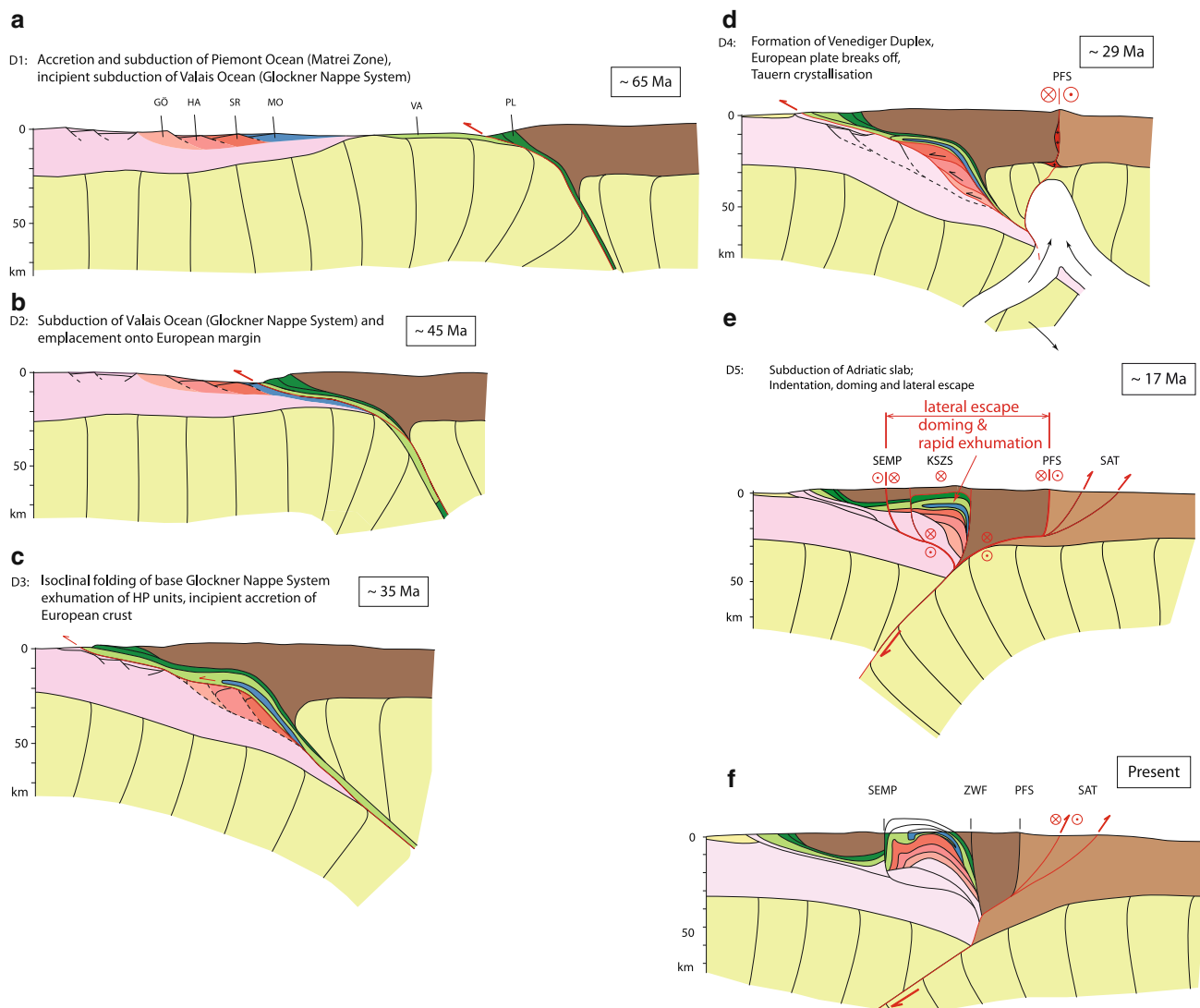
Fig. 6 Sketches illustrating the tectonic evolution of the Tauern Window. a D1 subduction of the Piemont-Liguria Ocean and accretion of oceanic relics in front of the Austroalpine nappe stack ( \approx 65 Ma, i.e. Cretaceous-Palaeogene boundary), abbreviations as follows: GÖ Göss nappe, HA Hochalm nappe, SR Sonnblick-Romate nappe, VA Valaisan (Glockner Nappe system), PL Piemont-Liguria (Matrei Zone); b D2 subduction of the Valais Ocean and parts of the distal European margin ( \approx 41 Ma, i.e. latest Lutetian); c D3 exhumation of the high-pressure units and incipient accretion of the
