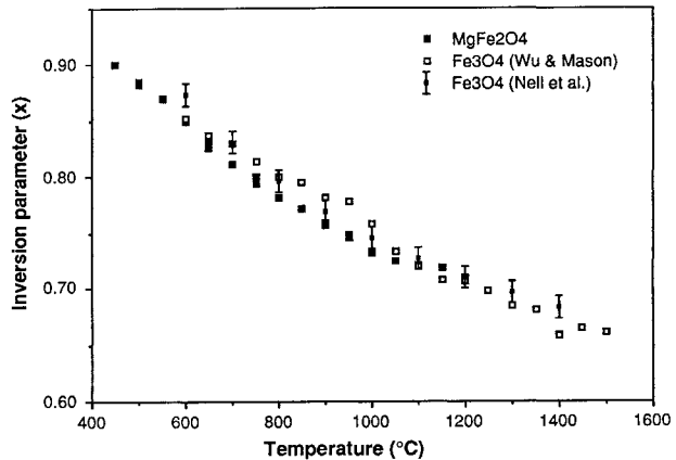
Fig. 13. Comparison of the temperature dependence of the cation distribution in quenched MgFe 2 O 4 , with that in Fe 3 O 4 measured at temperature, from the thermopower (Seebeck coefficient). Error bars for the thermopower measurements of Nell et al. (1989) are plotted as \pm 0.01 in x , which is approximately 25% of the uncertainty estimated by these authors. The internal consistency of the data and comparison with the measurements of Wu and Mason (1981) indicate that the original estimate is too pessimistic.
