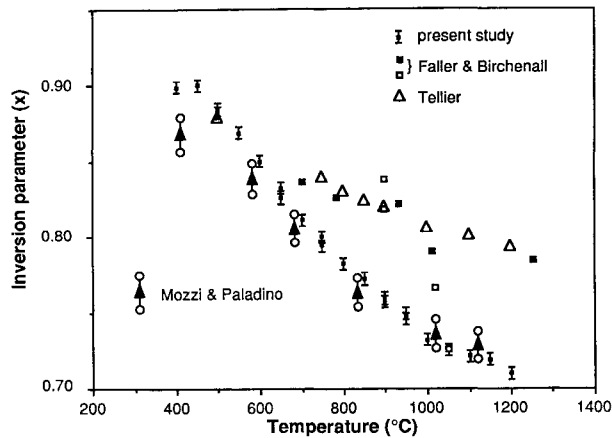
Fig. 12. Comparison of the present results on the inversion in MgFe 2 O 4 as a function of temperature with some previous results. For simplicity, only the present XRD results (from the Rietveld refinements) are shown. The XRD results of Faller and Birchenall (1970) on both quenched specimens (filled squares) and at temperature (open squares) are shown. The data of Mozzi and Paladino (1963) are shown both as reported (lower circles) and recalculated assuming stoichiometry (upper circles, connected to lower by an arrow). Their results, when corrected, coincide with the present study from 600 to 850 °C (they are plotted displaced along the temperature axis, for clarity), with their datum at 410 °C falling below the curve, and their data at 1000 and 1100 °C above, as do also the a_0 values for these experiments—see Figure 4.
