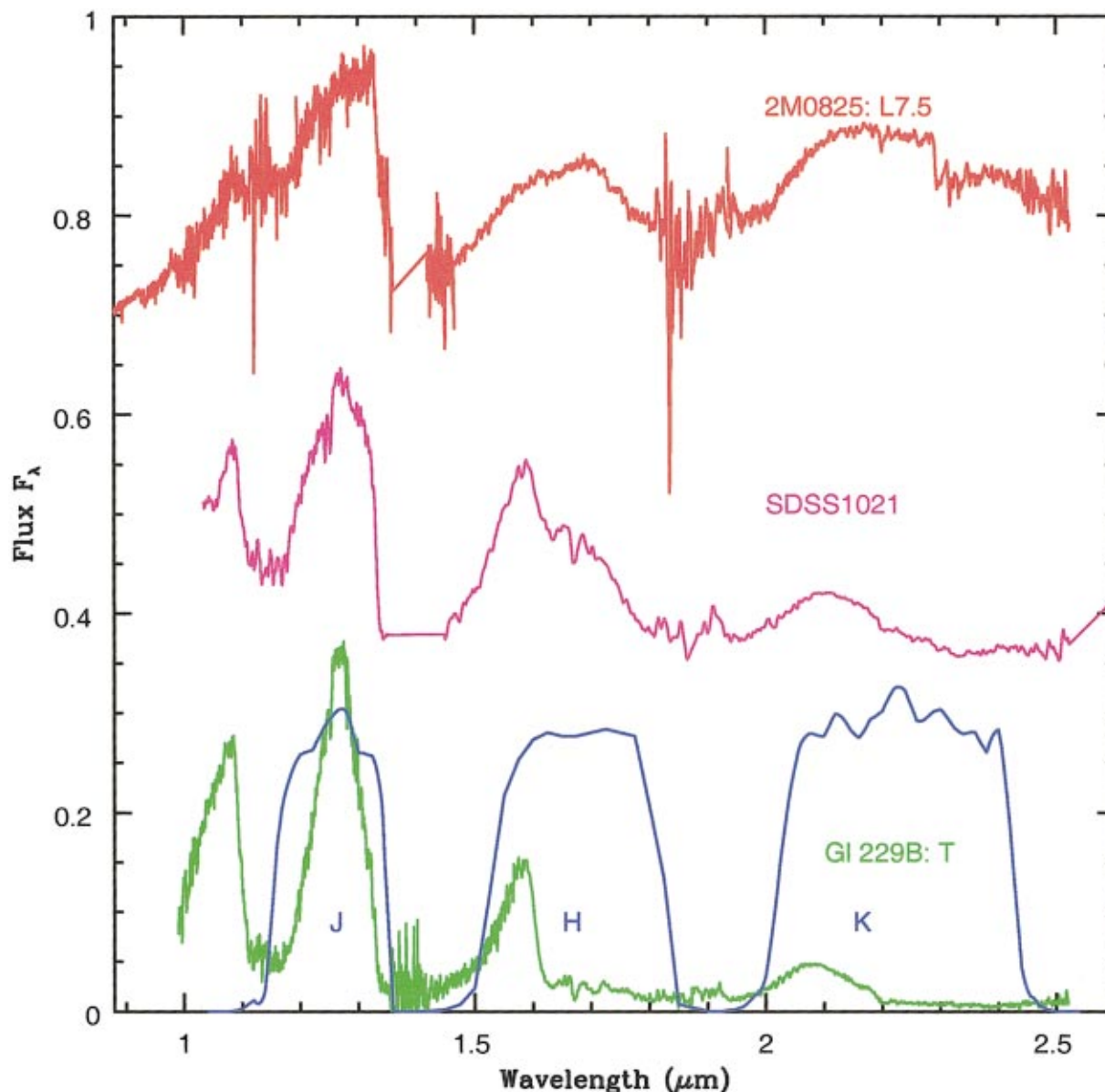
FIG. 23. The transition from L to T in near-infrared spectra courtesy of S. Leggett and I. N. Reid (private communication). Data for GI 229B are taken from Geballe et al. (1996). Superposed are the nominal response curves for the J (1.2 \mu\text{m} ), H (1.6 \mu\text{m} ), and K (2.2 \mu\text{m} ) photometric bands [Color].
