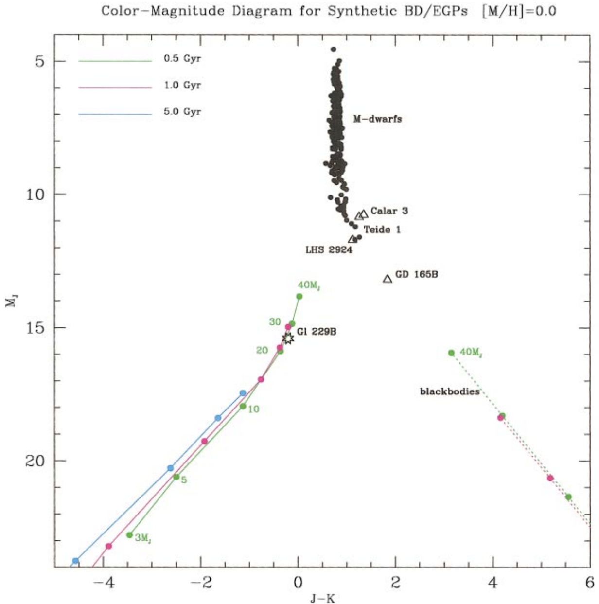
FIG. 24. Absolute J vs J-K color-magnitude diagram. Theoretical isochrones are shown for t=0.5, 1, and 5 Gyr, along with their blackbody counterparts. The difference between blackbody colors and model colors is striking. The brown dwarf Gliese 229B, the L dwarfs Calar 3, Teide 1, and GD 165B, and the very late M dwarf LHS 2924 are plotted for comparison (Kirkpatrick, Henry, and Simons, 1994, 1995; Oppenheimer et al. 1995; Zapatero-Osorio, Rebolo, and Martin 1997). The lower main sequence is defined by a selection of M-dwarf stars from Leggett (1992). Figure taken from Burrows et al. (1997) [Color].
