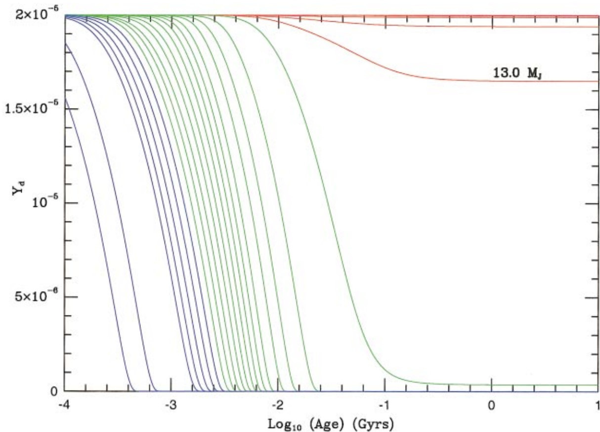
FIG. 6. The evolution due to thermonuclear burning of the deuterium mass fraction for various models of substellar-mass objects for the same mass set as listed in Fig. 1. The initial deuterium mass fraction assumed was 2 \times 10^{-5} . As indicated in the figure, the 13 M_J model is the lowest-mass model to show appreciable deuterium burning. Moreover, the more massive models burn deuterium more quickly and more completely. See Secs. II and IV for details [Color].
