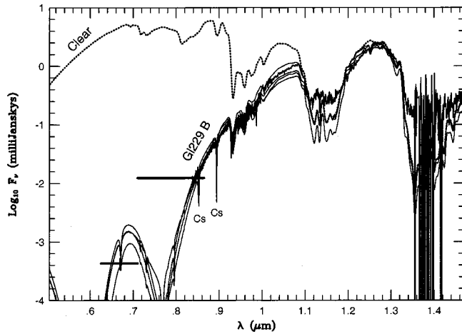
FIG. 27. The log of the absolute flux ( F_\nu ) in milliJanskys vs wavelength ( \lambda ) in microns from 0.5 to 1.45 \mu\text{m} for Gliese 229B: heavy solid line, according to Leggett et al. (1999); light solid lines, four theoretical models described in Burrows, Marley, and Sharp, 2000. Also included is a model, denoted “Clear” (dotted), without alkali metals and without any ad hoc absorber due to grains or haze. The horizontal bars near 0.7 and 0.8 \mu\text{m} denote the WFC2 R and I band measurements of Golimowski et al. (1998). From Burrows, Marley, and Sharp, 2000.
