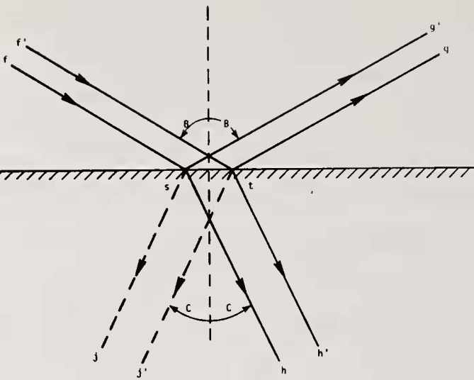
Figure 3. Reflection and refraction at plane interface.
