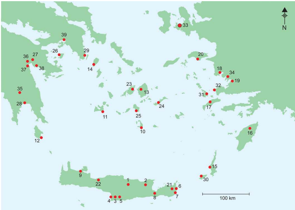
Figure 1. The Aegean, showing the 39 sites selected for the generation of the maritime network. Important sites, for the discussion that follows, include Knossos (1) and Thera (10). The remainder are listed in Table 1. The outline of the Thera caldera is shown.
