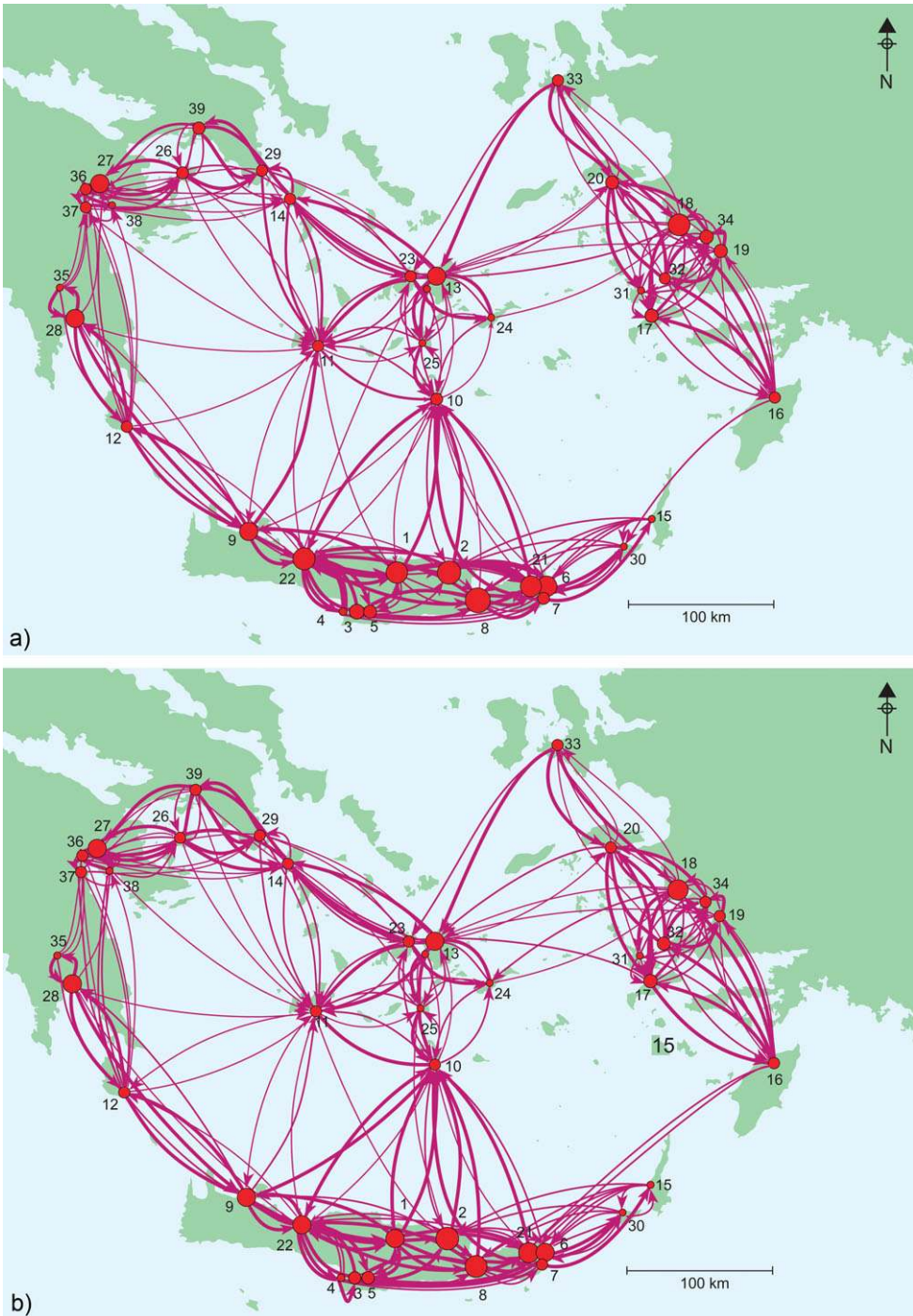
Figure 2a–b. Two exemplary runs of the model for the identical parameter values \lambda = 4 , \kappa = 1 , \mu = 0.1 , j = -2 , d = 110 (see Technical Appendix for more detail). The size of the nodes, the site weights, reflects the respective ‘population’ and the thicknesses of the lines, the link weights, reflects the annual traffic along them. In each case the importance of Thera as a link between Crete and the rest of the Aegean is clearly visible.
