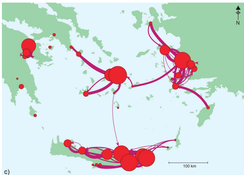
Figure 4a–c. Three exemplary runs of the model in which, beginning from the parameter values \lambda = 4 , \kappa = 1 , \mu = 0.1 , j = -2 , d = 110 of Figure 3, we increase the costs of sustaining links, implemented by increasing the parameter \mu (see Technical Appendix).
