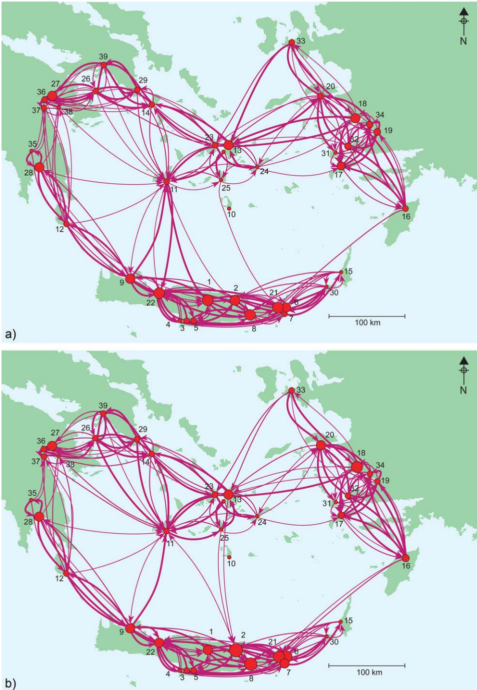
Figure 3a–b. Two exemplary runs of the model for the identical parameter values \lambda = 4, \kappa = 1, \mu = 0.1, j = -2, d = 110 (as in Figure 2) on removing Thera from the network. With regard to both weight and rank Knossos and N. Crete dominate. For impact, Kasos, Zakros, Kalymnos, Knossos, and then N. Crete are most important in Figure 3a, Kasos, Karpathos, Kalymnos, Zakros and N. Crete in Figure 3b. Total population and Trade are essentially unchanged from pre-eruption averages.
